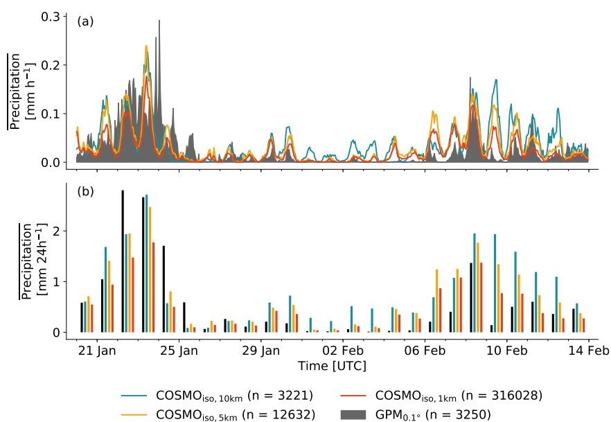
Figure 8. Time series displaying (a) hourly and (b) daily domain-averaged precipitation. Shown are the values from \text{COSMO}_{\text{iso},10\text{km}} (teal), \text{COSMO}_{\text{iso},5\text{km}} (yellow), \text{COSMO}_{\text{iso},1\text{km}} (red), and GPM (black). Only the data in the domain 54.5\text{--}61^\circ \text{W} , 11\text{--}16^\circ \text{N} are taken into account. The number of grid points in the domain is given in brackets.
