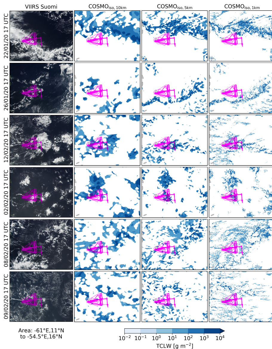
Figure 4. Spatial organisation of the clouds in the domain 54.5–61° W and 11–16° N from four datasets (columns) and on six dates (rows). The first column shows the image from the VIIRS instrument on board the polar-orbiting Suomi-NPP satellite (approx. equatorial crossing time 17:30 UTC). The remaining columns show the total column cloud liquid water (TCLW) in the three COSMO iso simulations at 17:00 UTC. The dates are chosen according to the displayed cloud species, with large/small Fish clouds on 22/26 January 2020, large/small Flower clouds on 12/2 February 2020, and Gravel-Sugar/Sugar clouds on 8/9 February 2020. The track from all ATR flights is overlaid in pink. Other examples are shown in Supplement 1.
