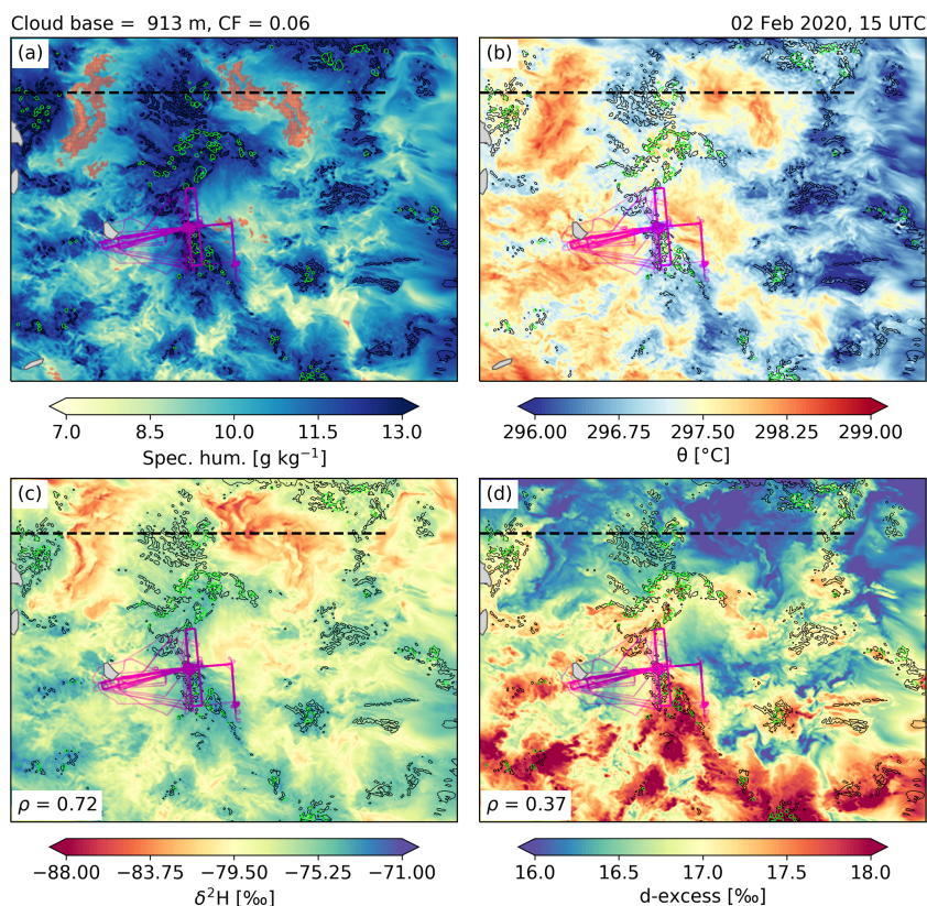
Figure 13. Fields of (a) specific humidity, (b) potential temperature, (c) \delta^2\text{H} in vapour, and (d) d -excess in vapour at cloud base ( z = 913 m) in the domain 54.5\text{--}61^\circ W and 11\text{--}16^\circ N from the COSMO iso,1km dataset at 15:00 UTC on 2 February 2020. The transparent red dots in panel (a) show grid points identified as dry-warm (see definition in text); the pink lines represent the track from all ATR flights; and the black line indicates the position of the cross-section shown in Fig. 14. Liquid cloud water contents of 10\text{ mg kg}^{-1} are shown as black contours and rain water contents of 1\text{ mg kg}^{-1} as green contours. In panels (c, d), the Pearson correlation coefficients ( \rho ) between the cloud base specific humidity and (c) \delta^2\text{H} in vapour, (d) d -excess in vapour are indicated in the lower left corner. The cloud base cloud fraction (CF) at this time and in this region corresponds to 6 %.
