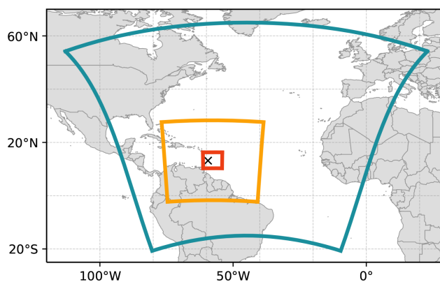
Figure 2. Domain boundaries of the three COSMO_{iso} simulations, i.e. COSMO_{iso,10\text{ km}} (teal), COSMO_{iso,5\text{ km}} (orange), and COSMO_{iso,1\text{ km}} (red). The location of Barbados is indicated by a black cross.
