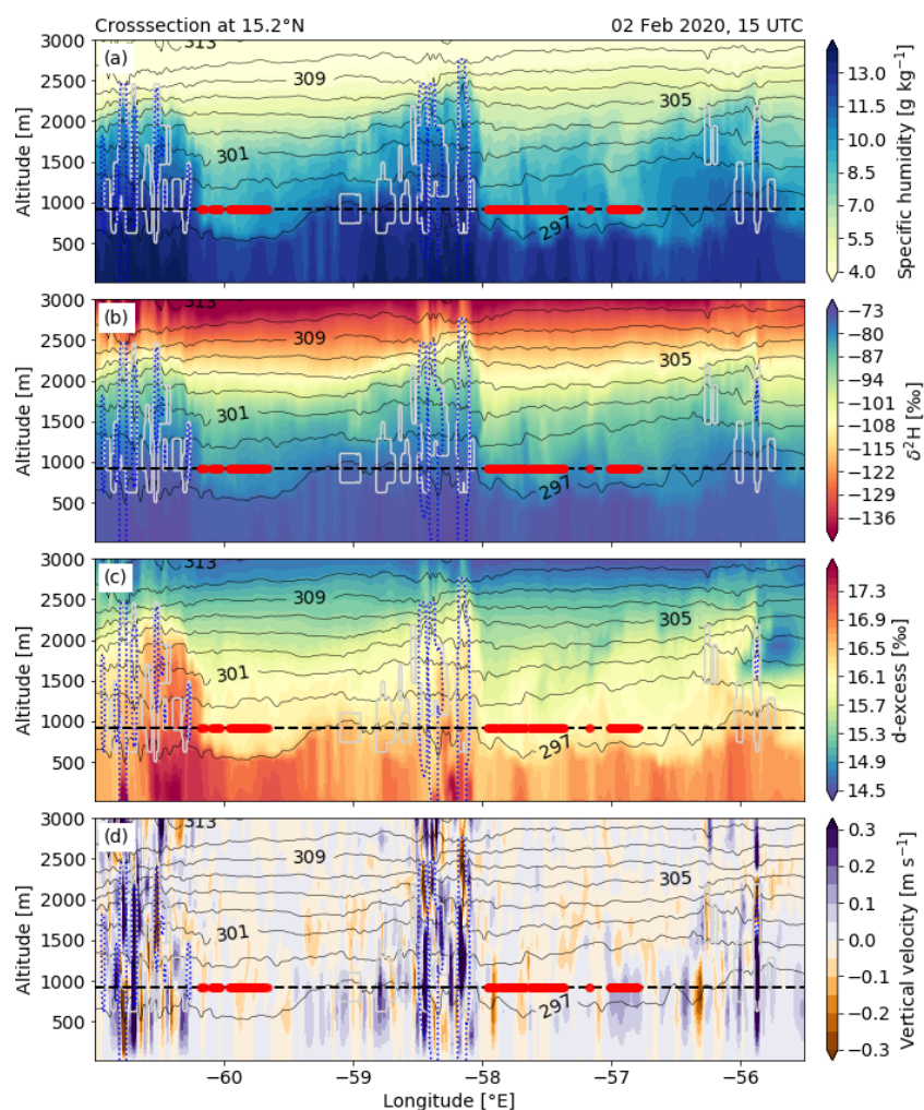
Figure 14. Cross-sections at 15.2° N of (a) specific humidity, (b) \delta^2\text{H} in vapour, (c) d -excess in vapour, and (d) vertical velocity from COSMO iso, 1 km at 15:00 UTC on 2 February 2020. Shown is also potential temperature (black contours), cloud water contents of 10 mg kg −1 (grey contours), rain water contents of 10 mg kg −1 (dashed blue contours) and cloud base height (dashed black line; the level at which the fields are shown in Fig. 13) with the cloud base grid points identified as dry-warm (red dots; less than 0.01° latitude away from the cross-section). The location of the cross-section is indicated in Fig. 13.
