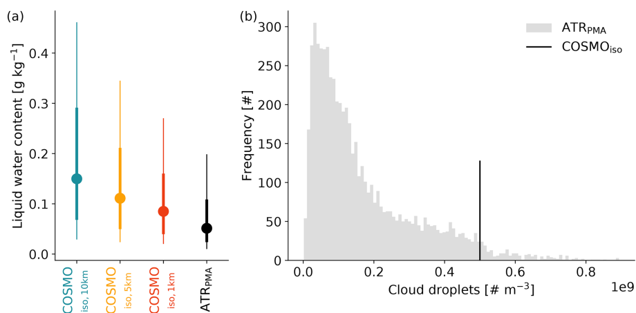
Figure 6. Distributions at cloud base of (a) liquid water content (LWC) from COSMO iso,10km (teal), COSMO iso,5km (orange), COSMO iso,1km (red), and ATR PMA (black); and (b) cloud droplet numbers from COSMO iso (black) and ATR PMA (grey). For COSMO iso , the LWC is calculated as the sum of cloud water content (CWC) and rainwater content (RWC; that is, LWC = CWC + RWC ). Shown are (a) the 10th to 90th percentile range (thin vertical line), 25th to 75th percentile range (thick vertical line), and the median (marker) of all cloud base data points with LWC > 10 \text{ mg kg}^{-1} . For the ATR PMA dataset, all flights (RF02–RF20) are taken into account; for COSMO iso , the data in the domain 54.5–61° W and 11–16° N from the hourly time steps that are closest to the ATR flights are taken into account. In panel (b), the droplet number distribution from the ATR PMA dataset during time steps flagged as cloud is shown together with the constant cloud droplet number of the one-moment cloud scheme of COSMO iso .
