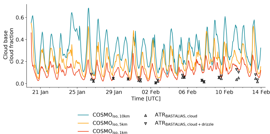
Figure 5. Time series of cloud fraction at cloud base for COSMO iso,10km (teal), COSMO iso,5km (orange), COSMO iso,1km (red), and the ATR (black markers). For COSMO iso , the cloud fraction is calculated as the fraction of cloud base grid points in the domain 54.5–61° W and 11–16° N with cloud water content exceeding 10 mg kg −1 . The number of grid points in the considered domain are 3221 for COSMO iso,10km , 12 632 for COSMO iso,5km , and 316028 for COSMO iso,1km .
