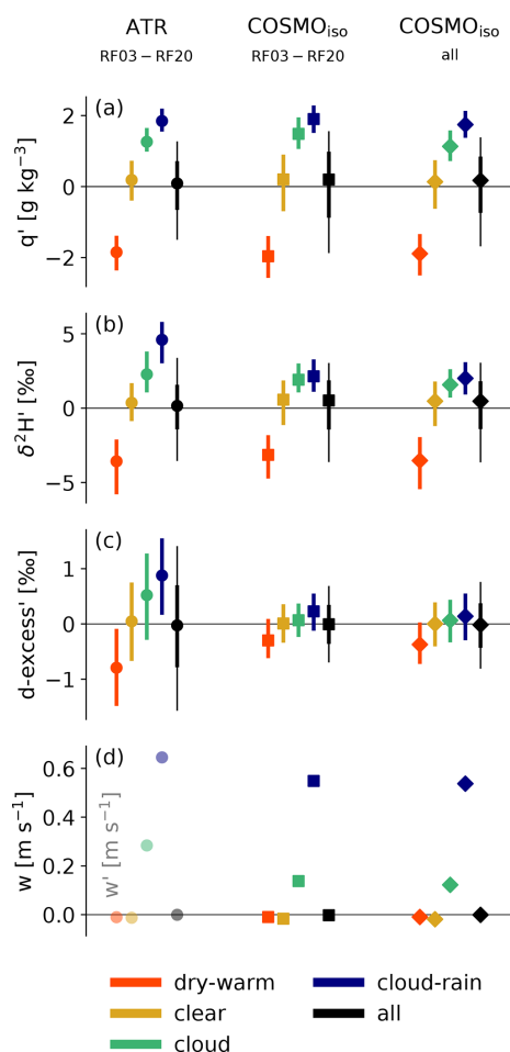
Figure 15. Distributions of the cloud base anomalies in (a) specific humidity, (b) \delta^2H in vapour, and (c) d\text{-excess} in vapour of the data points identified as dry-warm , clear , cloud , cloud-rain (see the text for the definition) and all of them together (black). For the ATR data, anomalies are defined relative to each flight's mean cloud base conditions. For COSMO iso,1 km , anomalies are defined relative to each time step's mean cloud base conditions in the domain 54.5–61° W and 11–16° N. Shown are the median (markers), the 25th to 75th percentile range (lines), and for the overall distribution (black) the 10th to 90th percentile range (thin black line) of the cloud base data points collected by the ATR (RF03–RF20) and the COSMO iso,1 km cloud base grid points at the hourly time steps that are closest to the ATR flights (COSMO iso,RF03–RF20 ) and over the whole simulated period (20 January to 13 February 2020; COSMO iso,all ). (d) The mean absolute vertical velocity w for COSMO iso and mean vertical velocity fluctuations w' for the ATR (see text for the reasoning behind the variable choice) at cloud base. For the ATR, only RF10–RF19 provide vertical velocity measurements and are included here. Table 4 gives the percentage of data points in each category and Table 5 gives the numerical values of the median anomalies. Supplement 3 provides alternative versions of this figure.
