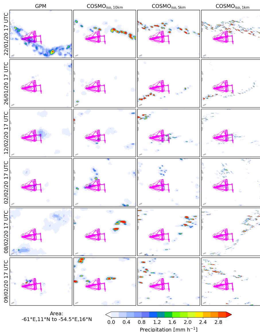
Figure 7. Hourly precipitation in the domain 54.5–61° W and 11–16° N from four datasets (columns) and on six dates (rows; also shown in Fig. 4). The first column shows the satellite-based precipitation estimate GPM (IMERG). The remaining columns show precipitation from the three COSMO iso simulations from 16:00–17:00 UTC.
