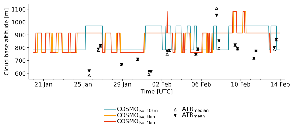
Figure 3. Time series of cloud base COSMO iso model level and ATR flight altitude. Shown are the median values of the grid points in the domain 54.5–61° W and 11–16° N at every hourly time step for COSMO iso,10 km (teal), COSMO iso,5 km (orange), and COSMO iso,1 km (red), as well as the median (empty black markers) and mean (filled black markers) value of each ATR flight.
