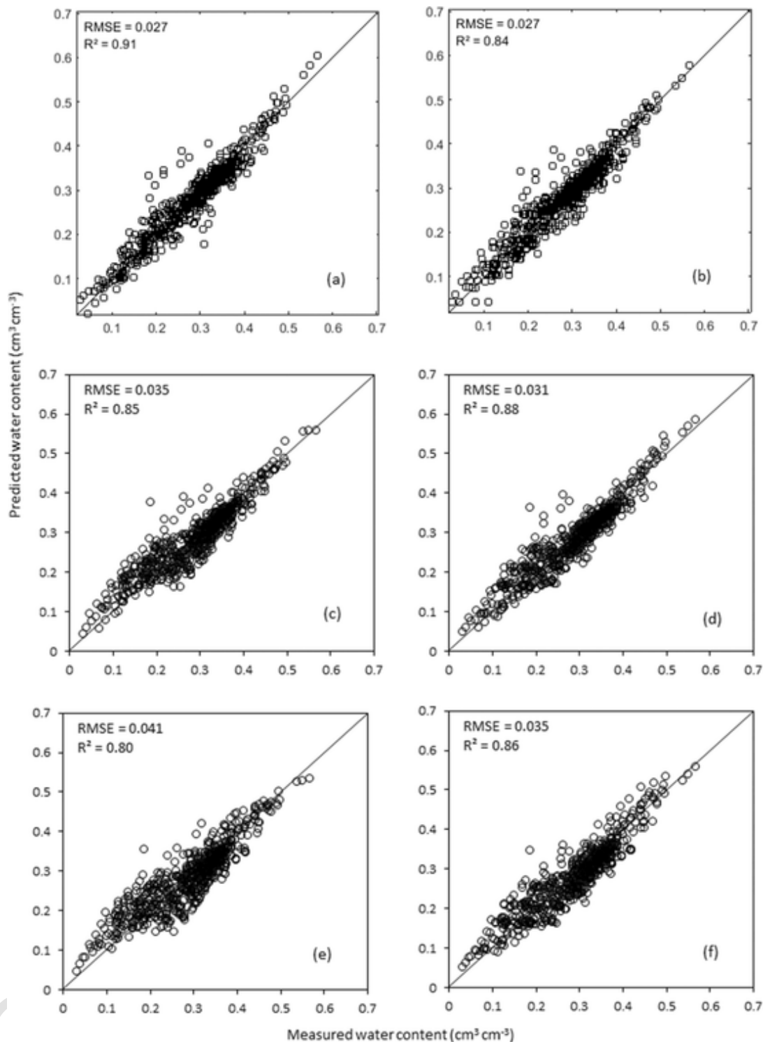
Fig. 2. Comparison of measured and predicted volumetric water content on the test dataset using ANN-PTFs with SC, BD_{FC}^p and \theta_{FC} as predictors (a), SVM-PTFs with SC, BD_{FC}^p and \theta_{FC} as predictors (b), SLR-PTFs with \theta_{FC} as predictor without any stratification (c), SLR-PTFs with \theta_{FC} as predictor after stratification by texture (d), SLR-PTFs with \theta'_{FC} as predictor without any stratification (e), SLR-PTFs with \theta_{FC} as predictor after stratification by texture (f).
