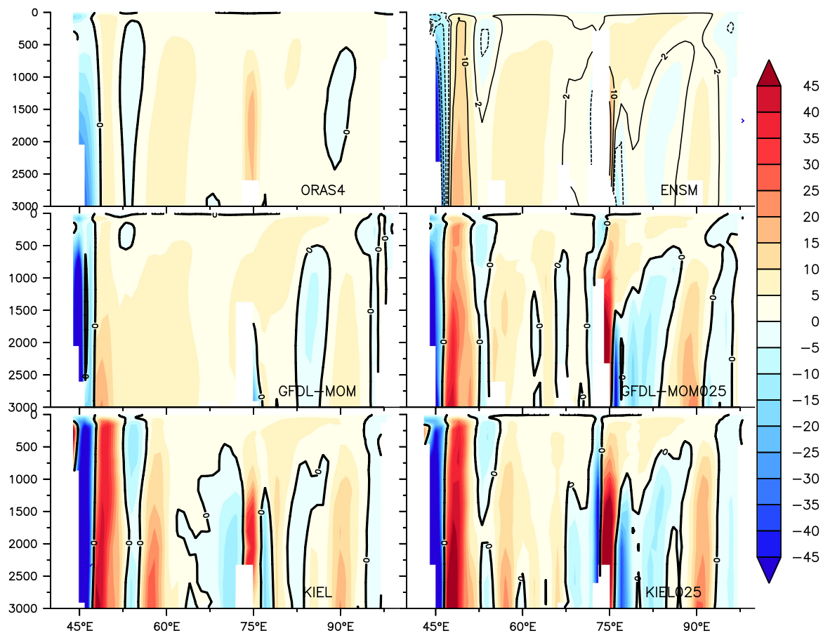
Fig. 32a. Transport across the equator from MOM, MOM25, KIEL, KIEL25, all model ensemble and ORAS4 in January. Units are in m^2/s .
