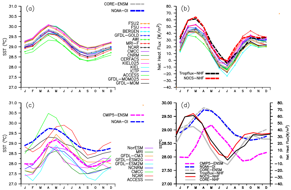
Fig. 12. Same as Fig. 10 but for the Eastern Equatorial Indian Ocean (EEIO).
