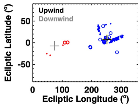
Figure 4. The distribution of observations relative to the upwind and downwind directions of the IPH flow, in ecliptic J2000 coordinates. Blue data points represent upwind observations made from IPH campaigns (open circles) and from limb scans (dots). Red data points represent downwind observations with similar symbols as used for upwind. The standard IPH upwind/downwind flow directions are shown as a black/gray crosses for reference.
