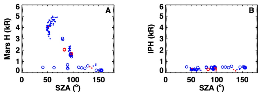
Figure 8. The variability of H emission brightness with solar illumination, denoted by solar zenith angle, derived from (a) Mars thermal atoms, and (b) Interplanetary atoms.
