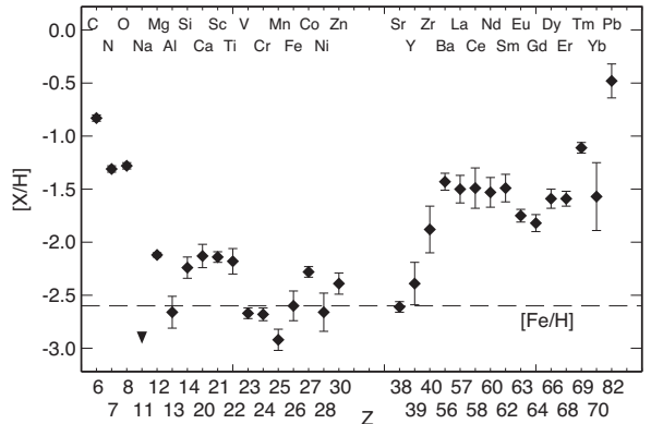
Figure 6. The element abundance pattern of Pr184237. An upper limit for the Na abundance is indicated by downward-facing triangle. The dashed line indicates the star's iron abundance [Fe/H] = -2.60 . Abundances of Cr, Mn, Co, and Ni are increased by 0.14 dex, see text for more details.
