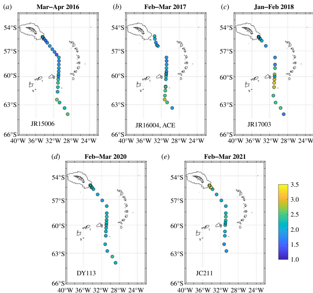
Figure 9. Percentage meteoric water at the surface from the cruises. Note in particular the relative invariance across the years, with the exception of 2021 very close to South Georgia ( e ). This was the time that the remnants of giant iceberg A68 were in the vicinity (figure 10), adding glacial melt to the ocean during its demise; this is seen in more detail in figure 11. Also of note are the elevated values above the South Scotia Ridge in early 2018. (Online version in colour.)
