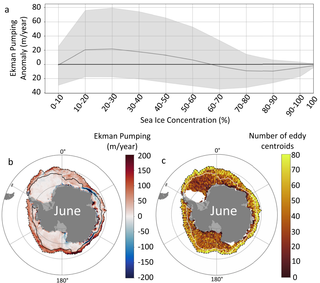
Figure 7. Ekman pumping and number of eddies detected in the ice-covered Southern Ocean. (a) Median Ekman pumping anomaly as a function of sea ice concentration ranges. (b) Mean Ekman pumping velocities in June in the ice-covered region of the Southern Ocean, between 2013 and 2019. (c) Number of eddies detected in 1^\circ pixel in the sea ice zone in June between 2013 and 2019. In (b and c), the dashed, and plain lines are respectively the contours of 10%, and 70% of Sea Ice Concentration.
