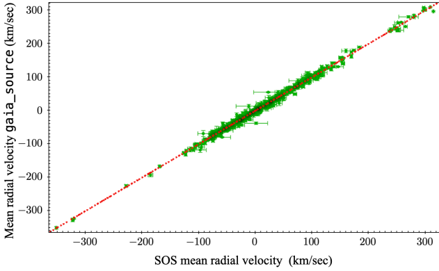
Fig. 12. Comparison between the average RV calculated by the SOS Cep&RRL pipeline from fitting the RV curves and the mean values published in the Gaia _source table (see Sartoretti et al. 2022, for details).
