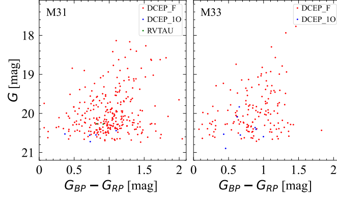
Fig. D.3. CMD in apparent G magnitude of the M31 (left panel) and M33 (right panel) Cepheid samples.
