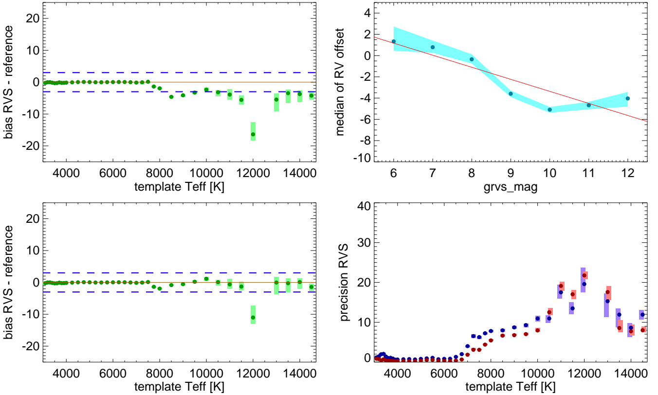
Fig. 6. Radial velocities compared to their reference values, where ReDetermineApHotStars has been applied to the hotter stars. Top left panel: bias of the radial velocity of the stars (RVS value minus reference value). It should be compared to the equivalent plot in Fig. 4 to see the improvement due to ReDetermineApHotStars. The dashed blue lines indicate \pm 3 \text{ km s}^{-1} . Top right panel: median of the radial velocity bias of stars in the T_{\text{eff}} = 8500\text{--}14\,500 \text{ K} range, binned in one-magnitude-wide (grvs_mag) bins. The relation between the two is fitted linearly (red line). Applying the magnitude-related correction leads to an improved set of radial velocities, which are once again compared to their reference values ( bottom left panel ). The precision of these improved values is shown in the bottom right panel . Similarly to Fig. 4, the blue symbols give the external precision, and the red symbols give the internal precision. All plots include only stars with grvs_mag \leq 12 mag.
