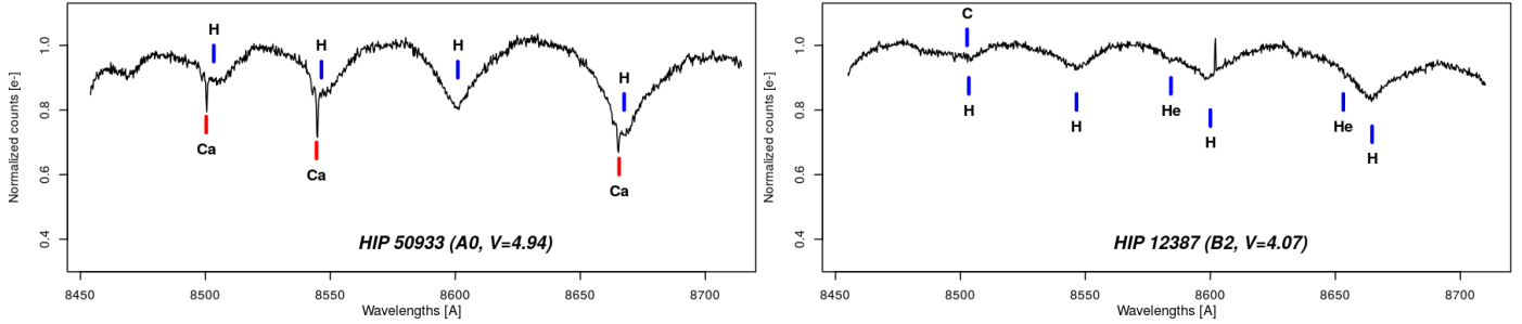
Fig. 1. Two examples of RVS spectra of hot stars ( https://www.cosmos.esa.int/web/gaia/iow_20141124 ). Both stars have Paschen hydrogen lines, and the cooler star ( left panel ) also shows the calcium infrared triplet lines. A spectrum of the cooler star with a much higher S/N is available in the DR3 archive ( Gaia DR3 1053778957742409984).
