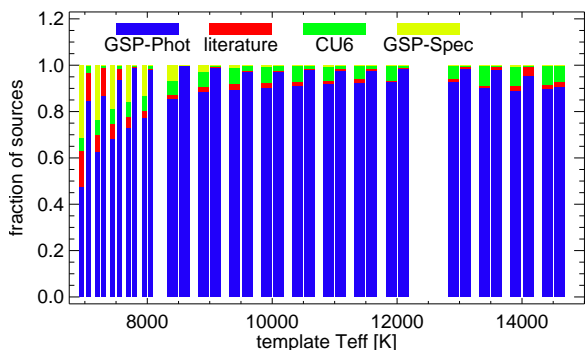
Fig. 3. Histogram showing the fraction of the stars that obtained their template parameters from the various input possibilities. The x -axis shows the template effective temperature. Each histogram bar is split into two parts: the left-hand side of each bar shows the distribution for \text{grvs\_mag} \leq 12 mag, and the right-hand side of each bar is for \text{grvs\_mag} > 12 mag.
