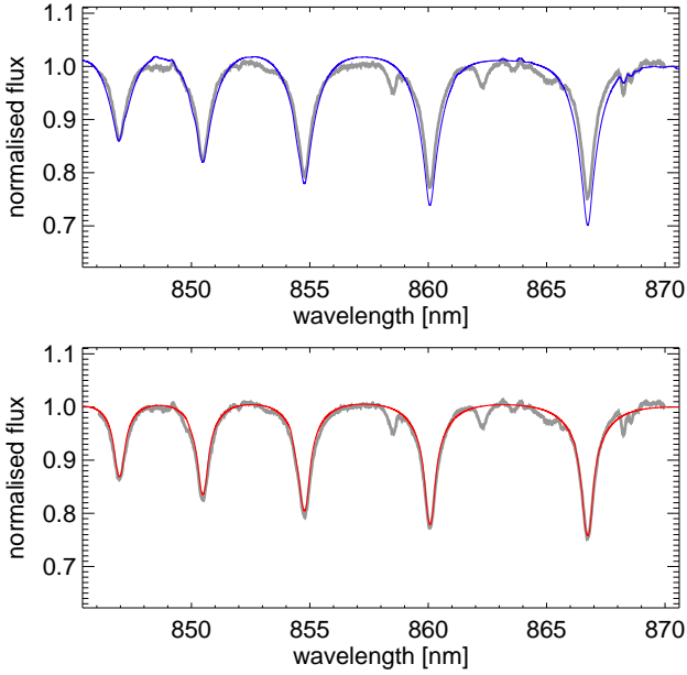
Fig. 8. Degeneracy between T_{\text{eff}} and metallicity for HDE 250290. Top panel: fit of the observed spectrum (grey) with a template (blue curve) corresponding closely to the parameters of Simón-Díaz et al. (2017, T_{\text{eff}} = 16\,000\text{ K} , \log g = 2.5\text{ dex} , [M/H] = 0.0\text{ dex} , and line-broadening velocity v_{\text{broad}} = 50\text{ km s}^{-1} ). Bottom panel: fit with the template (red curve) as determined by ReDetermineApHotStars ( T_{\text{eff}} = 6750\text{ K} , \log g = 2.5\text{ dex} , [M/H] = -5.0\text{ dex} , and v_{\text{broad}} = 80\text{ km s}^{-1} ).
