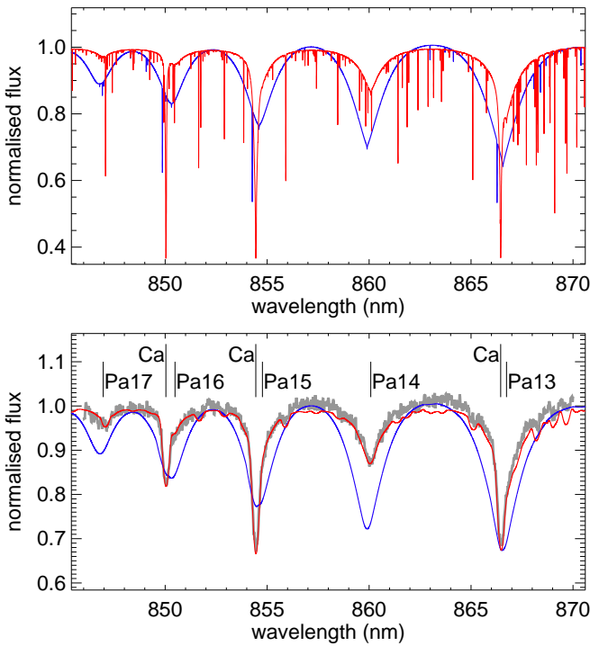
Fig. 5. Example of applying ReDetermineApHotStars. Top panel: shows the synthetic spectra: the blue curve ( T_{\text{eff}} = 11\,500\text{ K} , \log g = 4.0\text{ dex} , [M/H] = -0.50\text{ dex} ) presents data to which ReDetermineApHotStars was not applied, and the red curve shows the best synthetic spectrum as determined by ReDetermineApHotStars ( T_{\text{eff}} = 7750\text{ K} , \log g = 4.5\text{ dex} , [M/H] = +0.25\text{ dex} ). Bottom panel: the templates derived from these synthetic spectra: they have been convolved with a broadening velocity of 100\text{ km s}^{-1} (blue curve), and 80\text{ km s}^{-1} (red curve), and with the instrumental profile. They are compared with the observed spectrum of Gaia DR3 51853419339515136 (grey curve). All spectra are at their vacuum rest wavelength, except for the blue curves, which are shifted by -60.9\text{ km s}^{-1} ; this is the offset we found between the case when ReDetermineApHotStars was applied or was left unused. The template selected by ReDetermineApHotStars (red curve) clearly provides a better fit to the observed spectrum and therefore also gives a more correct radial velocity.
