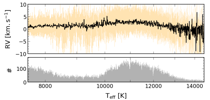
Fig. 7. Radial velocity shift that had to be applied by ESP-HS in CU8 to align the theoretical spectrum to the observed RVS spectrum as determined by MTA. It is plotted as a function of the T_{\text{eff}} determined by ESP-HS. Top panel: running median (computed over consecutive T_{\text{eff}} bins of 10 K) and the interquartile dispersion (15.85%–84.15%) of this offset as a function of the effective temperature. Bottom panel: how many stars went into each 10 K bin.
