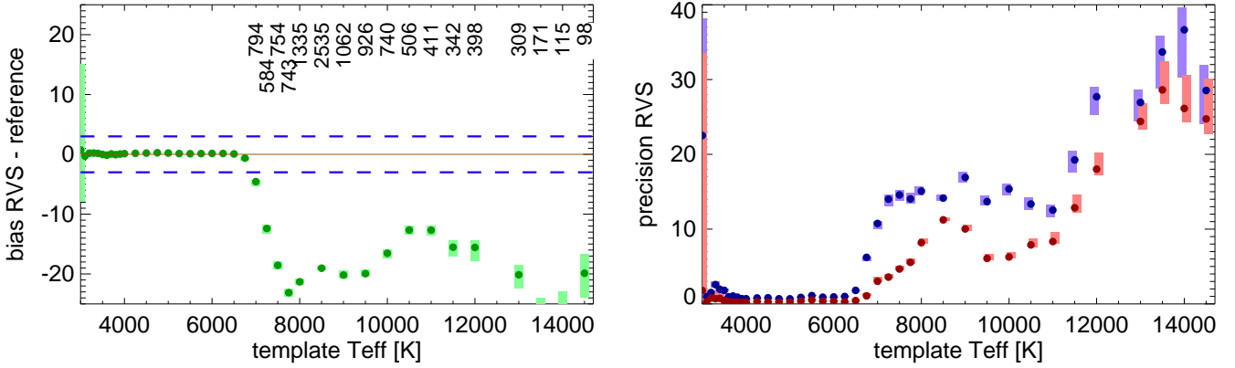
Fig. 4. Preliminary radial velocities compared to their reference values as a function of the template effective temperature. ReDetermineApHotStars was not applied to these data. Left panel: bias of the radial velocity of the stars (RVS value minus reference value). Each point on the plot presents the median of the bias of all stars having this T_{\text{eff}} value (the template effective temperatures take on only discrete values). The coloured bar around it gives the uncertainty on the median; in most cases, this uncertainty is smaller than the symbol. The results for cooler stars are also included in this figure to show the difference in quality of the radial velocity determination. The dashed blue lines indicate \pm 3 \text{ km s}^{-1} . The numbers at the top show how many stars correspond to this temperature. Right panel: precision. The blue symbols give the external uncertainty (dispersion of RVS value minus reference value), while the red symbols give the internal precision, i.e., the intrinsic uncertainty as derived by the code. The uncertainties on these values are given by the coloured bars; for the higher T_{\text{eff}} values, they have been offset slightly in temperature to avoid overlap. The plots include only stars with \text{grvs\_mag} \leq 12 \text{ mag} .
