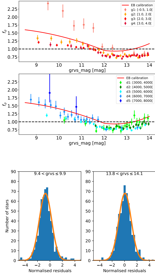
Fig. 8. From top to bottom, row 1: standard error factor (see text) as a function of grvs\_mag magnitude for the giant star samples. The range of surface gravity of each sample is provided in the legend. The red curve corresponds to the calibration of f_{\sigma} provided in Babusiaux et al. (2023). Row 2: same as row 1 for the dwarf star samples. The range of effective temperature of each sample is provided in the legend. Row 3: distributions of the normalised residuals of two groups of stars from the g2 giant sample (see Appendix E), selected in the magnitude ranges grvs\_mag \in [9.4, 9.9] (left) and [13.8, 14.1] mag (right). Gaussian profiles with standard deviations equal to 1 are overlaid (orange curves).
