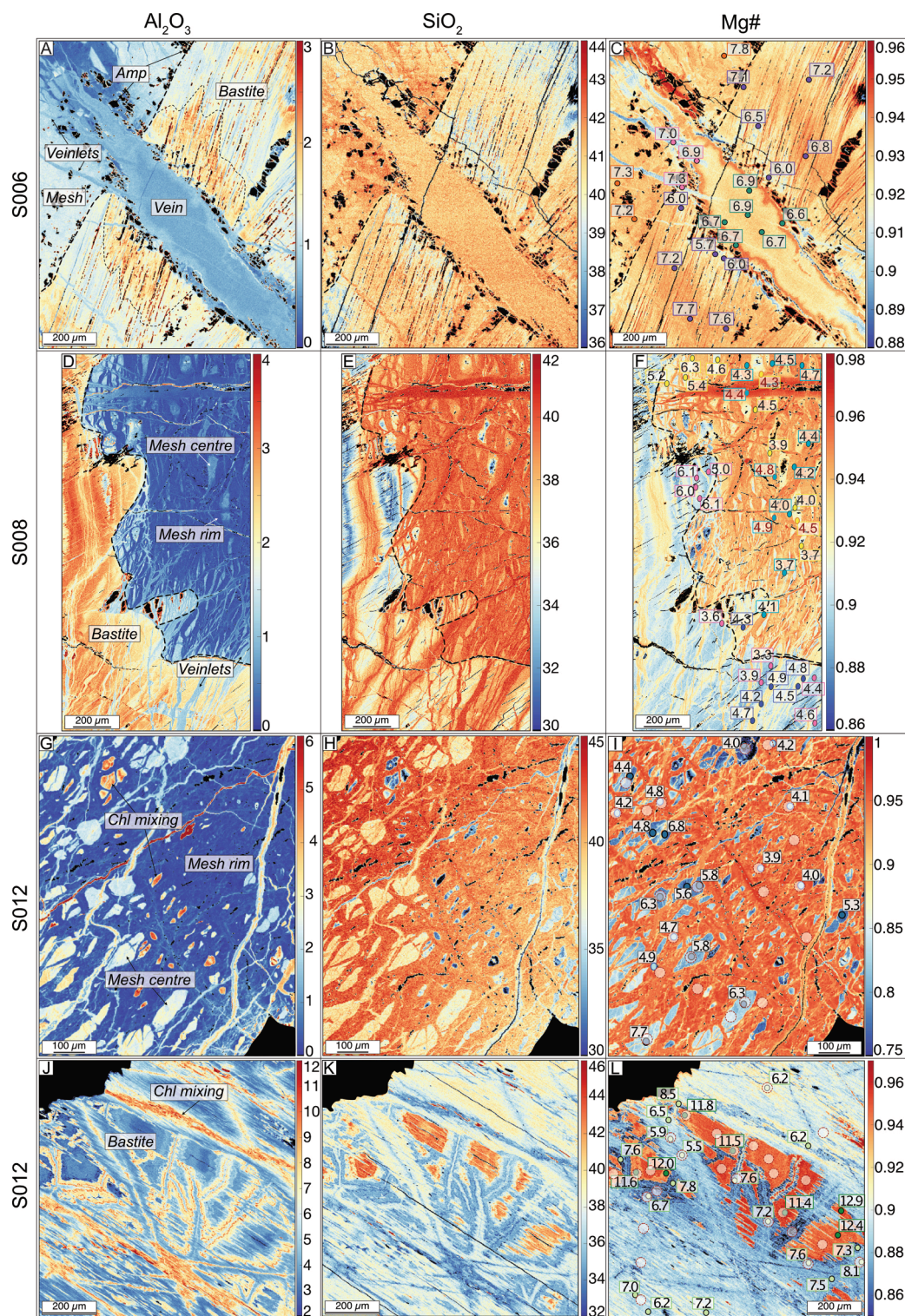
Fig. 2. Quantitative maps of serpentine for wt.% \text{Al}_2\text{O}_3 and \text{SiO}_2 , and Mg#. (A–C) Mesh, bastite and vein in sample S006 (Newfoundland). The black areas are amphiboles that were intentionally left out of the chemical maps. The zone of the bastite affected by the vein is highlighted with the black dotted line in map (A). (D–F) Bastite and mesh in sample S008 (Iberia). Note that the distinction between mesh rim and mesh centre was not visible in BSEimage (Fig. 1E), but is revealed by chemical maps. The black zones are pyroxene in the bastite domain, and magnetite in the mesh and bastite domains. Low Si domains in the mesh centre are due to porosity (E). (G–I) Mesh texture, both rim and centre in sample S012 (Iberia). The Al-rich zones can result from a mixing of serpentine with chlorite (G), or an Al-rich serpentine, consistent with low Si concentration in these zones. The black zones are magnetite (in the mesh network) and calcite (bottom right). (J–L) Zoned bastite in sample S012 (Iberia). The Al-rich zones are either due to the mixing of serpentine with chlorite, or an Al-rich serpentine, consistent with low Si content. The black zone on the top left corner is a calcite vein. The location of SIMS and LA-ICP-MS spots is shown on the Mg# maps, as well as the corresponding \delta^{18}\text{O} values in‰. Note that the Mg# maps consider all Fe as FeO.
