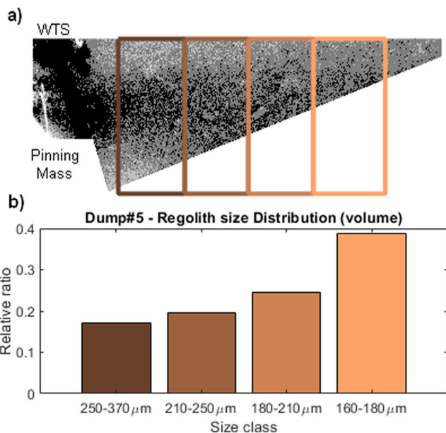
Figure 23. Grain size distribution for dump #5. Same legend as Figure 20, picture width represents 1.95 m. Wind speed is 7 \text{m.s}^{-1} .
