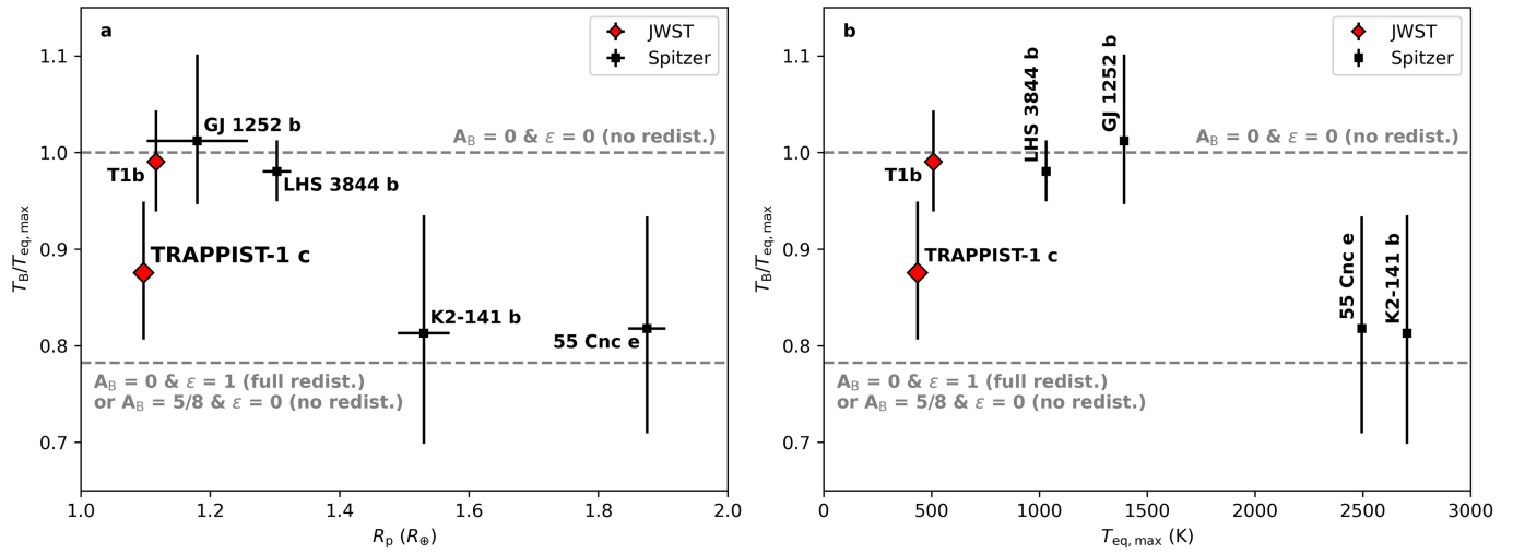
Extended Data Fig. 1 | Comparison of small exoplanets with measured infrared emission. Following ref. 8, we show the normalized dayside brightness temperature for super-Earths ( R_p < 2R_{\oplus} ) with measured thermal emission, as a function of planet size (a) and maximum equilibrium temperature (b). The brightness temperatures are normalized relative to predictions for a bare rock with zero albedo and zero heat redistribution,
