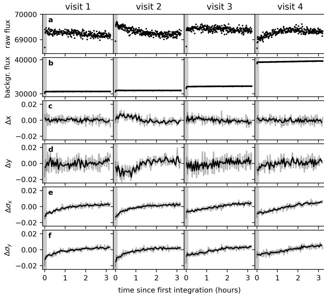
Extended Data Fig. 3 | Diagnostic plot of all four visits taken during JWST General Observer programme 2304 based on the SZ reduction. Every column corresponds to a visit. a, b , The top and second rows show the raw and background flux in units of electrons per integration per pixel, respectively. The raw flux is referring to the flux level within the target aperture before the subtraction of the background flux. c–f , The following rows are depicting the properties of the centroid over time. We fitted a 2D Gaussian distribution to the target at
