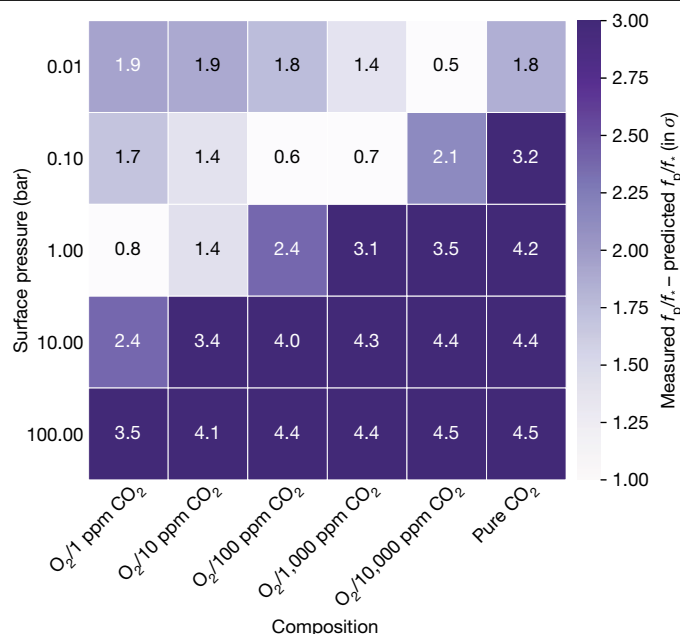
Fig. 2 | Grid plot comparing a suite of atmospheric models to the measured eclipse depth. Comparison between the measured eclipse depth and a suite of different O 2 /CO 2 , cloud-free atmospheres for TRAPPIST-1 c with varying surface pressures and compositions. Darker grid cells indicate that we more strongly rule out this specific atmospheric scenario. The number in each cell is the difference between each model and the observations in units of \sigma . The lower the modelled atmosphere is in the grid, the higher its surface pressure. The rightmost column shows pure CO 2 atmospheres. The other columns are O 2 -dominated atmospheres with different amounts of CO 2 , ranging from 1 ppm (=0.0001%) to 10,000 ppm (=1%).
