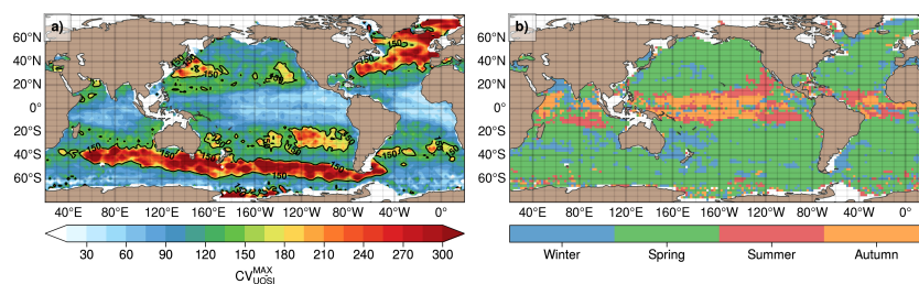
FIGURE 9 (A) Maximum coefficient of variation for the stratification index UOSI and (B) the corresponding season.
