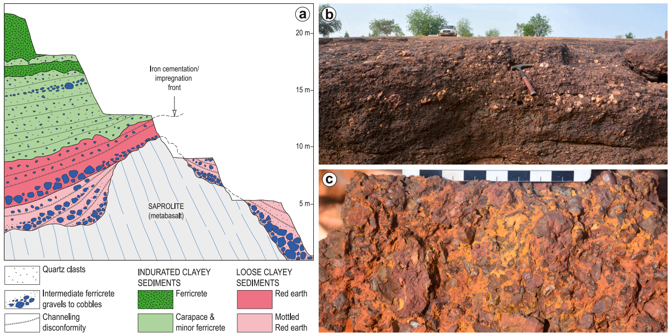
Fig. 12. Illustrations of relict Neogene piedmont pediment material (High and Middle glaciis) such as found in Residual Composite Topography (RT) terrains or around small isolated massifs in relict and zonal pediplain environments. (a) Sketch roadcut section through stacked debris flows of a High glaciis relic (Bondoukou area, Northeastern Côte d'Ivoire; coordinates: 8.18709°N/2.93752°W). Sediments are reworked weathering profiles filling up gullies >10 m deep. Sedimentologic structures are erased up-section as duricrusting increases, so that the topping ferricrete has no recognizable detrital character (comparable to that of Fig. 13a). (b) Middle glaciis conglomeratic ferricrete, Kongoussi area, Goren greenstone belt, Central Burkina Faso. Light-colored clasts are bauxites and darker cobbles are Intermediate ferricretes and Fe-nodules. The matrix is a cemented gravel of Fe-nodules. (c) High glaciis conglomeratic ferricrete. Gravels (mostly angular) are pink bauxites (locally pisolithic) and Intermediate ferricretes and Fe-nodules, cemented by a mix of kaolinite-rich clays and Fe-oxides (same glaciis relic as in (a) but 5 km farther to the North; scale bar in cm). (For interpretation of the references to colour in this figure legend, the reader is referred to the web version of this article.)
