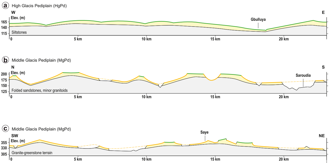
Fig. 13. Simplified cross-sections illustrating the landform-regolith associations of relict Neogene pediplains. Duricrusts are schematized as thick colored lines (green: High glaciis; orange: Middle glaciis); weathering mantles in yellow; geological substrate in grey. (a) High glaciis pediplain (HgPd), North-Central Ghana. Gbulluya village coordinates: 9.4865°N/1.0126°W. (b) Middle glaciis pediplain (MgPd), Southeasternmost Senegal. Sarouidia village coordinates: 12.5227°N/11.5780°W. (c) Middle glaciis pediplain (MgPd), Northwestern Burkina Faso. Saye village coordinates: 13.3021°N/2.2399°W. (For interpretation of the references to colour in this figure legend, the reader is referred to the web version of this article.)
