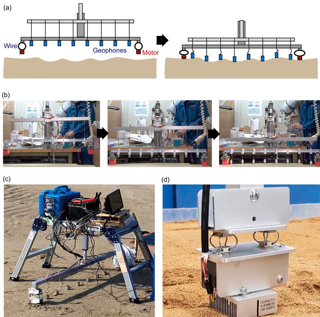
Fig. 1. Lunar Active Seismic Profiler (LASP). (a) Schematic diagram and (b) photos showing the operation of the LASP. (c) The LASP prototype during the field experiment (sand beach). (d) The portable active seismic source (PASS) deployed on the LASP. The wire cushion on top of the source provides a constant downward pressure and decreases the propagation of vibrations to the array frame.
