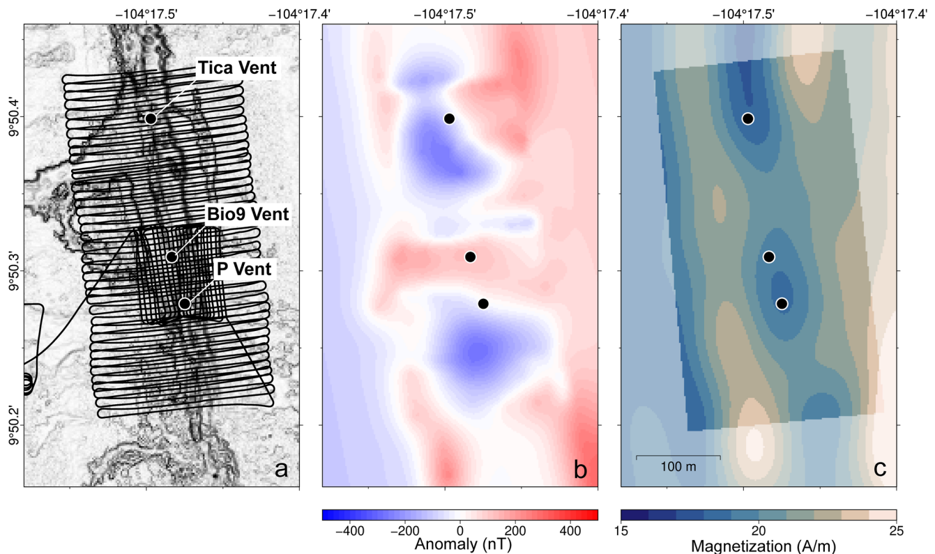
Figure 5. Near-bottom magnetic anomalies over axial summit trough and hydrothermal vents near 9°50.3'N. (a) Survey tracklines (black lines) and hydrothermal vent locations (black dots); survey lines spaced ~10 m, and ~25 m vehicle altitude enable detection of short-wavelength magnetic anomalies associated with hydrothermal vents. (b) Total field anomaly. (c) Total field crustal magnetization for an along-axis segment with hydrothermal vents, calculated with 135 m thick magnetic layer, corresponding to average layer 2A thickness in this region (Marjanović et al., 2018). Anomaly data were upward continued to 2,480 m, and filtered using a bandpass filter with 5 km and 80 m cutoffs. Twenty times a 1 A/m annihilator was added.
