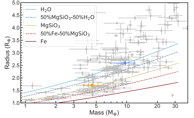
Figure 13. Mass-radius diagram plotted for TOI-836 b in orange and TOI-836 c in blue, with exoplanets from the TEPCAT catalogue (Southworth 2011) in grey and composition models from Zeng, Sasselov & Jacobsen (2016).
