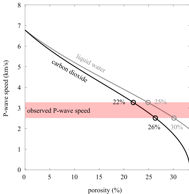
Figure 7. P-wave speed of porous basalt with intrusions of carbon dioxide (in black) and liquid water (in gray) as a function of porosity (with the aspect ratio of 0.1). The shaded red region marks the range of the average P-wave speeds from this study. The derived lower and upper limits for the porosity estimations are also indicated.
