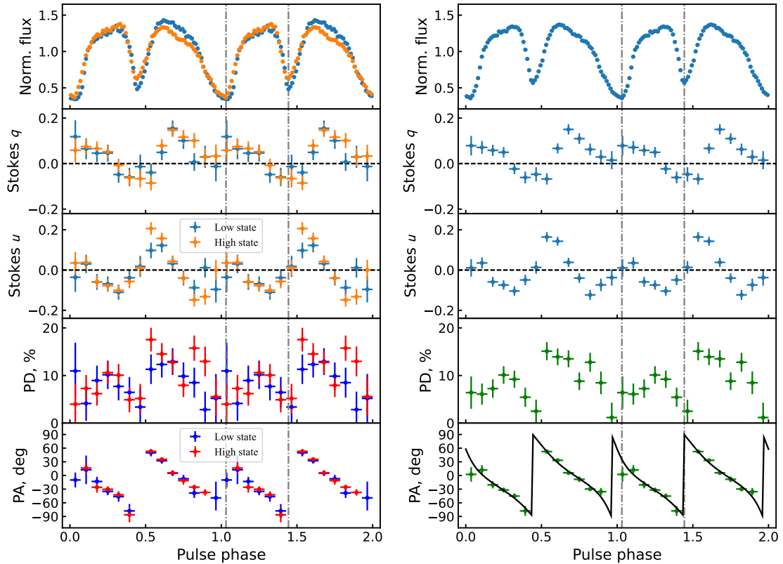
Fig. 4. Dependence of the normalized flux in the 2–8 keV energy band, normalized Stokes parameters q and u (based on the formalism by Kislak et al. 2015), PD, and PA (from the spectro-polarimetric analysis) on the pulse phase for two IXPE observations separately (left) and combined (right). Data from the three IXPE telescopes are combined. Vertical dash-dotted lines show the positions of two minima in the profile and are added for illustrative purposes. The black solid line in the bottom right panel shows the best-fit rotating vector model (see Sect. 4.2).
