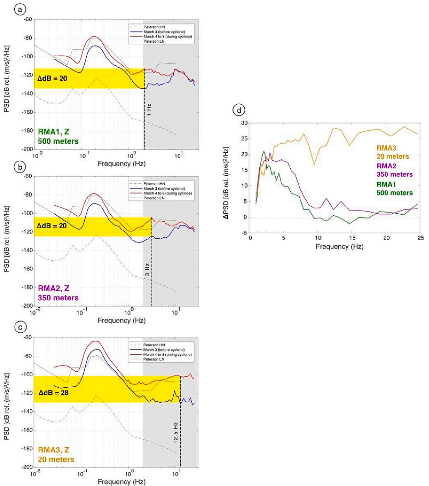
Fig. 4. a), b) and c) Average spectra calculated at RMA1, RMA2 and RMA3 respectively before the cyclone (March 3) in blue, and during the cyclone (March 4 to 8) in red, calculated with the SACPSD software (Herrmann, 2013). This representation allows the visualization of the noise variation induced by the cyclone and the flood, at the three sites and over the various frequencies. Solid black line represents the high noise (HN) level model whereas the dashed black curve shows the low noise (LN) level model from (Peterson, 1993). The grey part highlights the 2 to around 26 Hz frequency band. The dotted line indicates the frequency for which the \Delta PSD is maximum. d) Calculated difference in the noise spectra before and during the cyclone ( \Delta PSD ) for the three seismic stations in the frequency range 1 to 25 Hz, showing the different behaviour depending on the station distance to the riverbed. Note that RMA3 station, located closest to the river display variations of the seismic amplitude over the whole 1–25 Hz frequency band while the two other stations, located at larger distances show only variations in the low frequency band during the flood. (For interpretation of the references to colour in this figure legend, the reader is referred to the web version of this article.)
