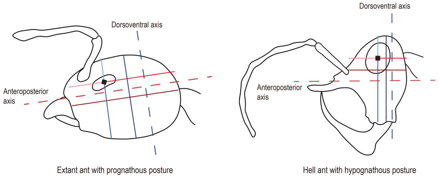
Figure S2. Eye positioning measurements consistent with functional morphology.
