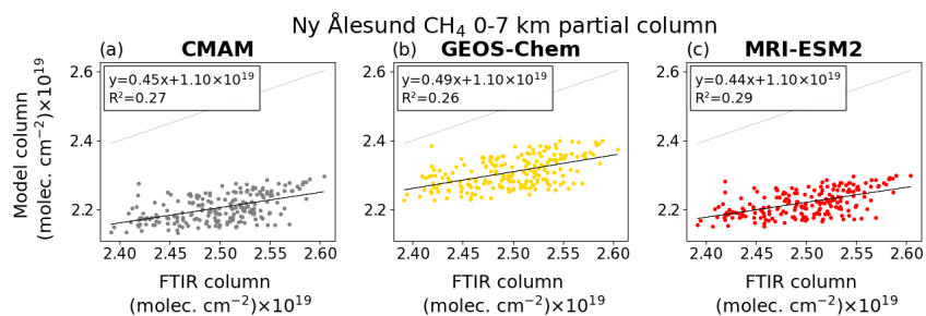
Figure A11. Smoothed model vs. FTIR 0–7 km partial column of \text{CH}_4 for Ny Ålesund, showing all available model–FTIR corresponding data. The black line is the line of best fit, where the equation and R^2 are noted in the legend. The 1 : 1 line is shown in light grey.
