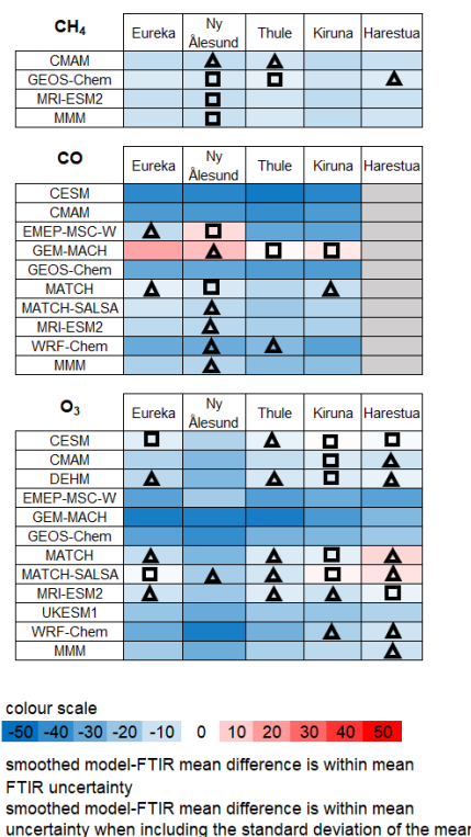
Figure 15. Summary of model–measurement mean percent difference ( \Delta_O ) for each model and location by species. MMM is the multi-model mean ( \Delta_{O,MMM} ). The colour scale indicates the mean percent difference relative to the FTIR measurements, from blue ( -50\% ) to red ( +50\% ). A square marker indicates that the mean percent difference is within the FTIR uncertainty. A triangle marker indicates that the mean difference is within the FTIR uncertainty combined with the standard deviation of the monthly mean percent difference.
