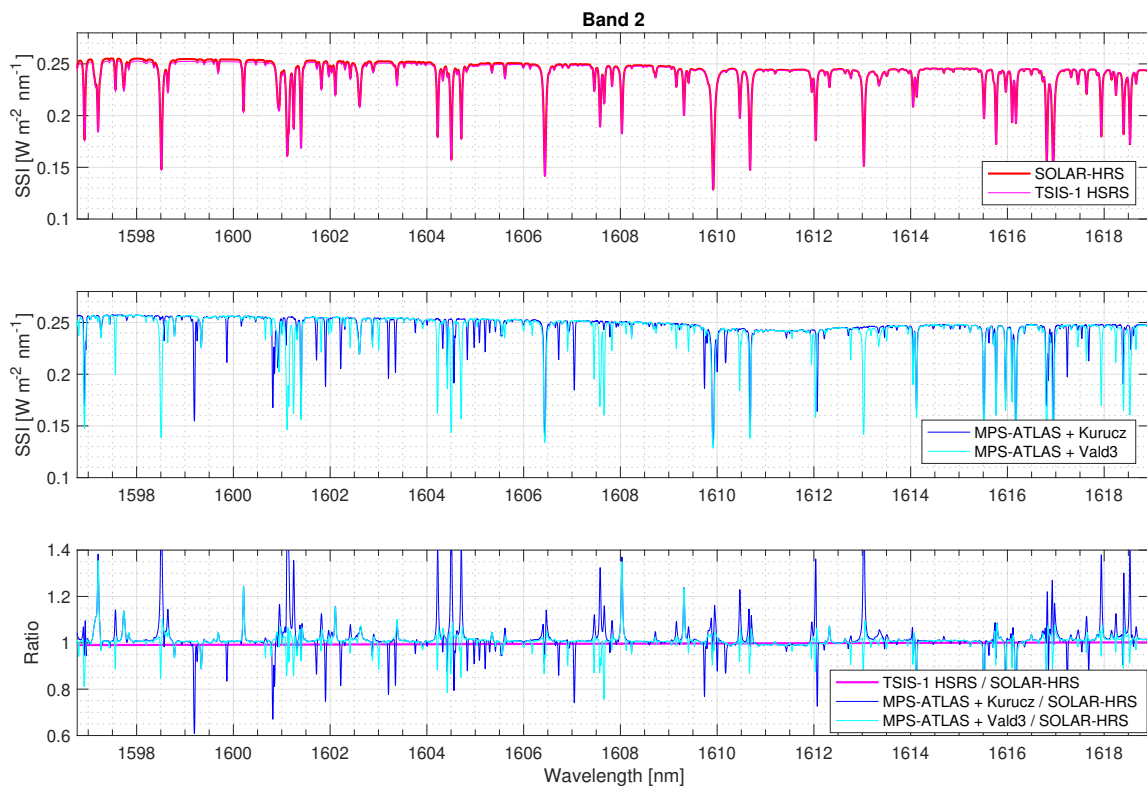
Figure 6. Disk-integrated SSI for SOLAR-HRS, TSIS-1 HSRS, and MPS-ATLAS—B2 band.
