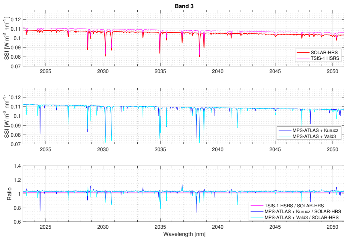
Figure 7. Disk-integrated SSI for SOLAR-HRS, TSIS-1 HSRS, and MPS-ATLAS—B3 band.
