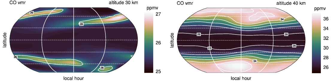
Figure 12. CO volume mixing ratio as modeled by Stolzenbach et al. (2023) at an altitude of 30 km (left) and 40 km (right). Dashed white lines indicate parallels (30° apart in latitude), and solid white lines indicate 6AM, noon and 6PM local solar times.
