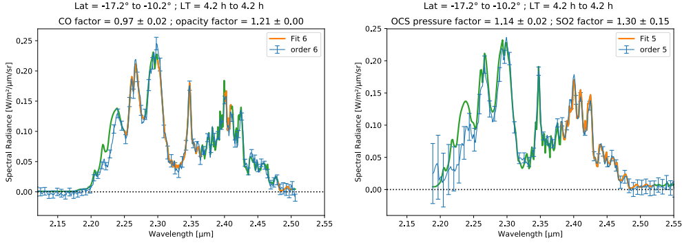
Figure 5. Best fits obtained during orbit # 277 for CO & cloud opacity with order 6 (left), and OCS & SO 2 with order 5 (right). Fitted intervals from Table 1 are shown in orange for the best fits, non-fitted intervals are shown in green for the best fits, and observed binned spectra along their 1\sigma error bars are shown in blue.
