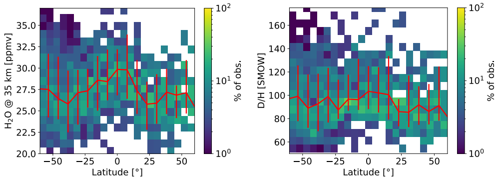
Figure 10. \text{H}_2\text{O} volume mixing ratio when assuming a constant D/H ratio of 130 (left) and D/H ratio assuming a constant water vapor mixing ratio of 30 ppmv (right) with respect to latitude. Color codes for the percentage of retrievals in the corresponding \text{H}_2\text{O} (left) and D/H (right) bin relative to all retrievals in the same latitudinal bin. The red curve and error bars represent the \pm 1\sigma statistical dispersion around the median.
