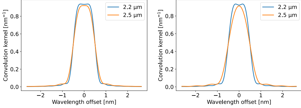
Figure 4. Normalized PSF shapes for order 5 (left) and 6 (right) for extremal wavelengths within the 2.3\ \mu\text{m} window.
