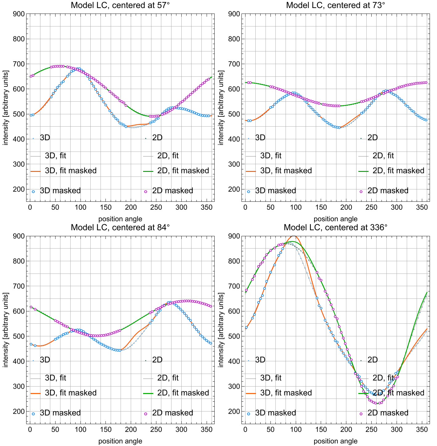
Figure 1. Model lightcurves for selected vantage locations. The model was calculated for the solar wind and EUV output characteristic for 2014, i.e., for solar maximum conditions. A comparison of lightcurves for spherically symmetric (“2D”) and latitudinally structured (“3D”) ionization rates is presented. Small dots represent lightcurves binned into 4^\circ bins along the scanning circle. Open circles represent the same quantities left after the application of SOHO/SWAN masks (see Figure 3). Solid lines represent fits of Equation (1) to full (thin lines) and masked (colored solid lines) lightcurves. The horizontal axis represents the position angle along the scanning circle counted off the northernmost point in the scanning circle. The numbers in the panel headers represent ecliptic longitudes of the centers of the scanning circles. The lower-right panel represents a vantage point close to one of the crosswind positions, where the max/min ratio for a lightcurve is the greatest. The other three panels represent a passage of the observer through the upwind longitude. The vantage locations were selected to correspond to those available in the SOHO/SWAN database (see Figure 6).
