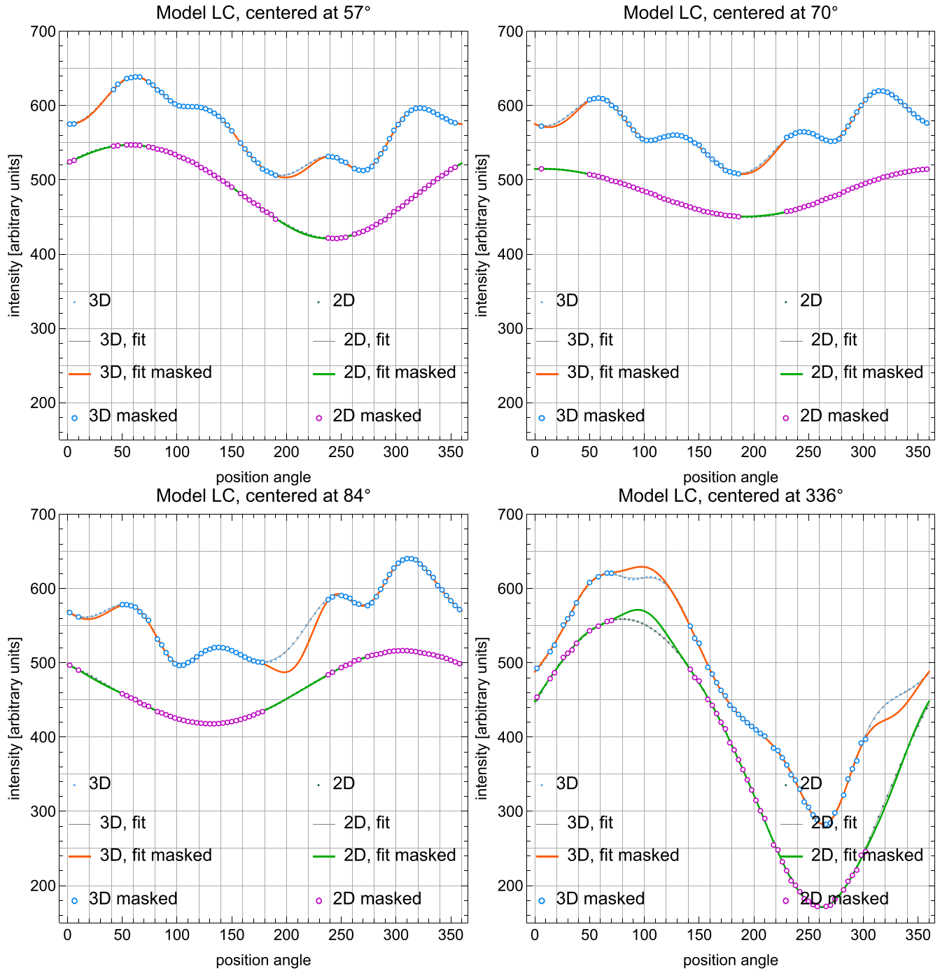
Figure 2. Similar to Figure 1 but for 2009, characteristic of solar minimum conditions.
