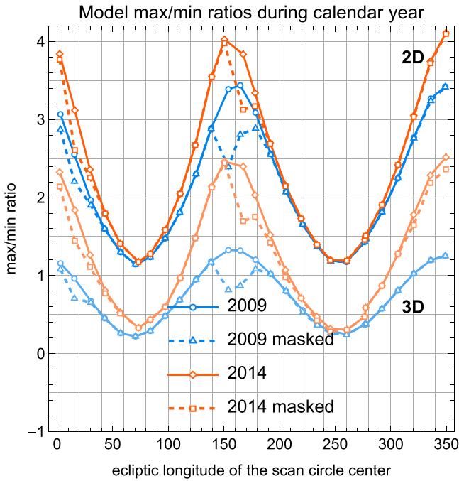
Figure 5. Variation of the max/min ratios of the helioglow intensities obtained for lightcurves simulated for individual vantage points distributed around the Sun during two selected calendar years, corresponding to solar minimum (2009) and solar maximum conditions (2014). Solid lines represent model ratios obtained for full simulated lightcurves, and broken lines those for simulated lightcurves with SOHO/SWAN masks applied. The upper set of lines marked as 2D and drawn using more vivid colors, represents the ratios simulated adopting spherically symmetric ionization rate. The lower set of lines, marked as 3D and drawn with pale colors, is offset by -1 relative to their native positions to improve the visibility. They represent the ratios simulated adopting latitudinally structured ionization rates.
