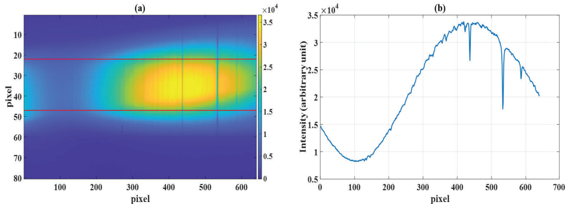
Figure 4. (a) Integration region in a diffraction order image. (b) Spectral band of the order corresponding to this integration region.
