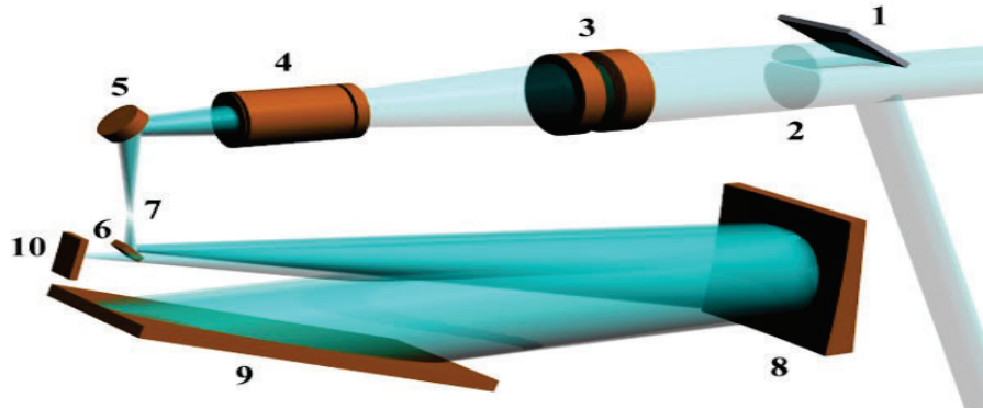
Figure 1. Optical scheme of the ACS-NIR spectrometer reproduced courtesy TGO-ACS.
