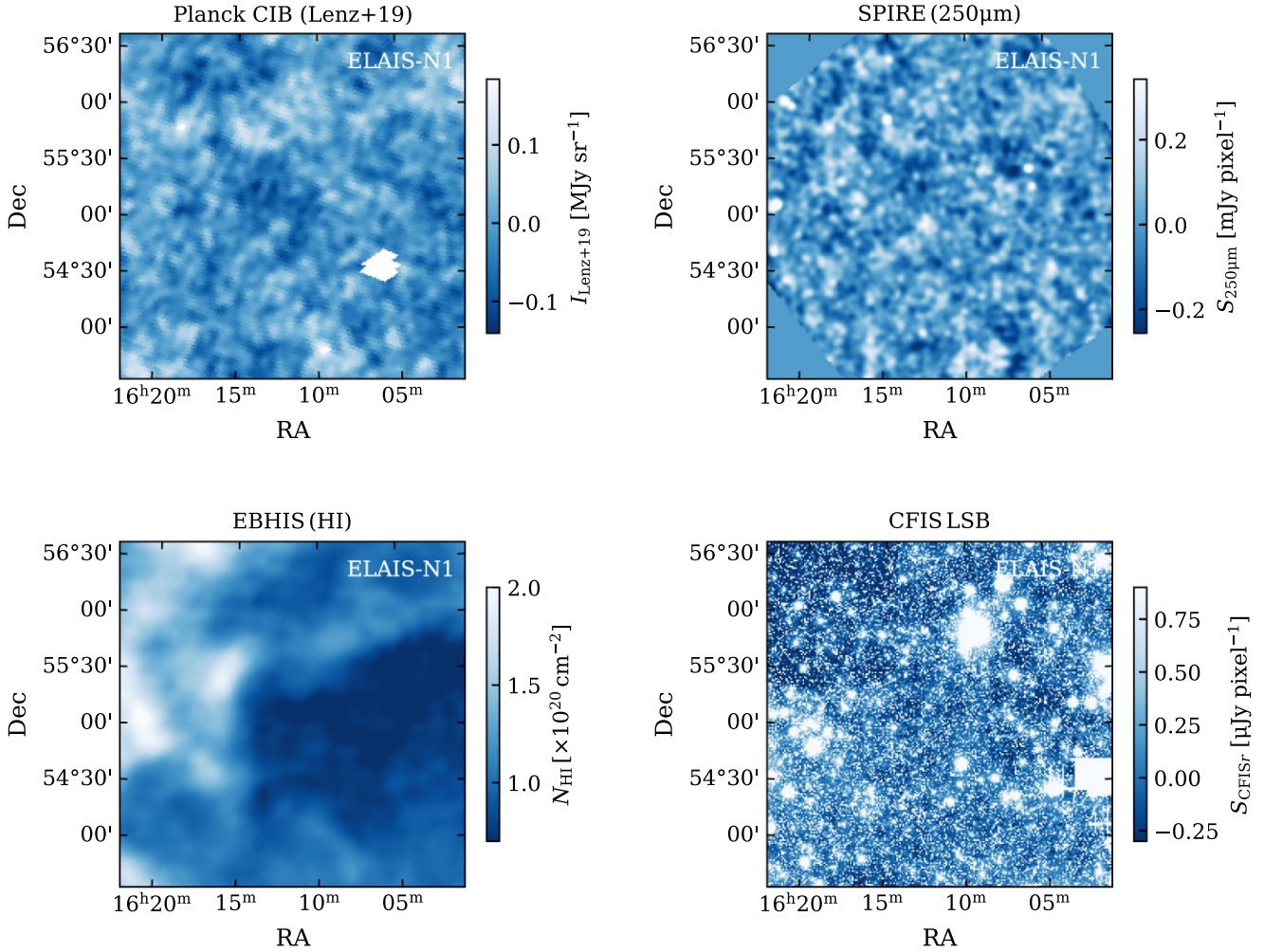
Figure 15. Visual comparison in the ELAIS-N1 field (as an example) between the SPIRE 250\ \mu\text{E} map, the Planck CIB map from Lenz et al. (2019), which is intended to show only the CIB component derived from Planck using a regression with HI surveys, EBHIS survey, and CFIS r -band LSB ‘B3 + MONTAGE’ version (galaxies are not masked). The strong visual agreement between the SPIRE and Planck map, in contrast to the much weaker correlation with the EBHIS, implies that fluctuations are dominated by the CIB rather than Galactic emission. In the bottom panels, the CFIS LSB map is also compared to the EBHIS map to present its correlation with the Galactic emission, although it is disturbed significantly by the bright individual sources.
