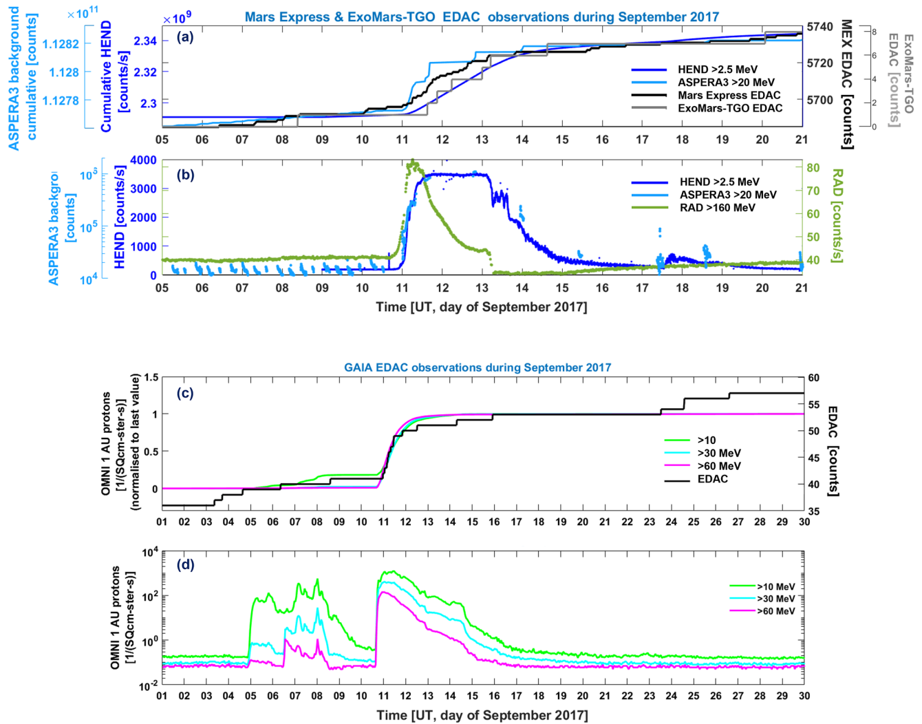
Figure 6. Solar particle event in September 2017. (a, b) Mars case. Mars Express (black) and ExoMars-TGO Error Detection and Correction (EDAC) observations together with cumulative sum (a) and count observations (b) of the solar particle event by ASPERA-3-Mars Express (light blue, y-axis in log-scale in panel b only) and High Energy Neutron Detector (HEND)-Mars Odyssey (dark blue) in orbit, and RAD-MSL at the surface of Mars (green). (c, d) Earth case. Gaia EDAC observations at L2 (black) together with cumulative sum (c) and flux observations (d) of three different energy bands of the solar particle event recorded at the OMNI data set at 1 au (note y-axis in log-scale).
