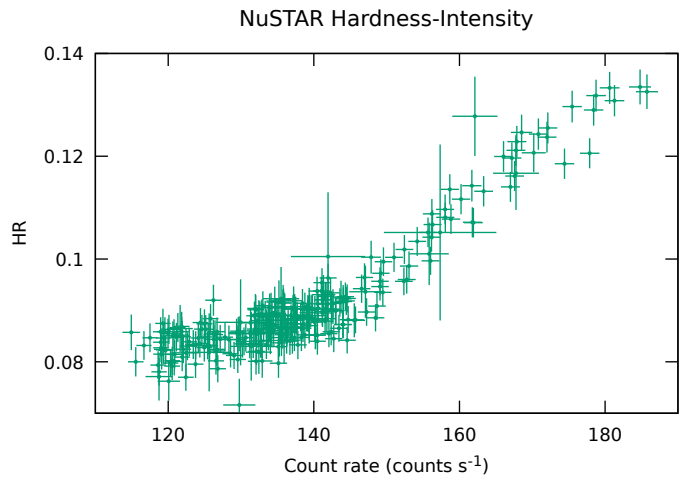
Fig. 3. NuSTAR count rate hardness ratio (10–30 keV/3–10 keV) vs. total count rate (3–30 keV). Time bins of 200 s are used.
