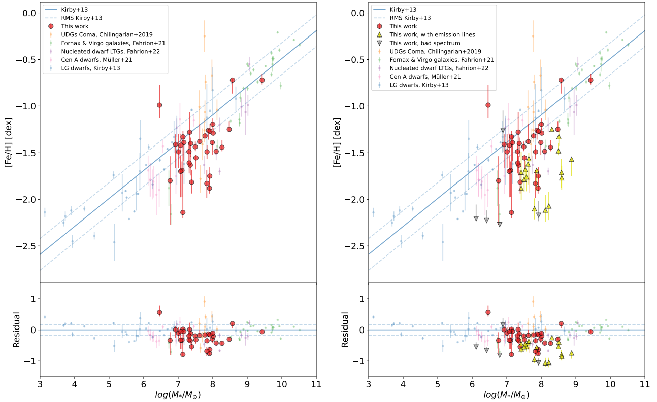
Fig. 10. Plot of universal stellar mass-metallicity relation from Kirby et al. (2013; blue solid line) with its rms (blue dashed lines). On the x -axis is plotted the logarithm of the stellar mass in units of solar mass. Left: data from this work (red circles), but excluding star forming and low S/N galaxies. Right: full sample from this work. Star forming galaxies are shown as yellow upward pointing triangles, while low S/N galaxies are gray downward pointing triangles. Shown is a comparison of our results with galaxies from other works: LG dwarfs (blue; Kirby et al. 2013), Cen A dwarfs (pink; Müller et al. 2021b), galaxies in Fornax and Virgo (green; Fahrion et al. 2021), nucleated dwarf LTGs (purple; Fahrion et al. 2022), and UDGs in the Coma cluster (orange; Chilingarian et al. 2019). Bottom: residual plots (i.e., metallicity dwarf-metallicity fit). The blue dashed lines indicate the rms of the fit from Kirby et al. (2013). The LG dwarf metallicities from Kirby et al. (2013) are iron metallicities ( [\text{Fe}/\text{H}] ), while all other data points show total metallicities ( [\text{M}/\text{H}] ).
