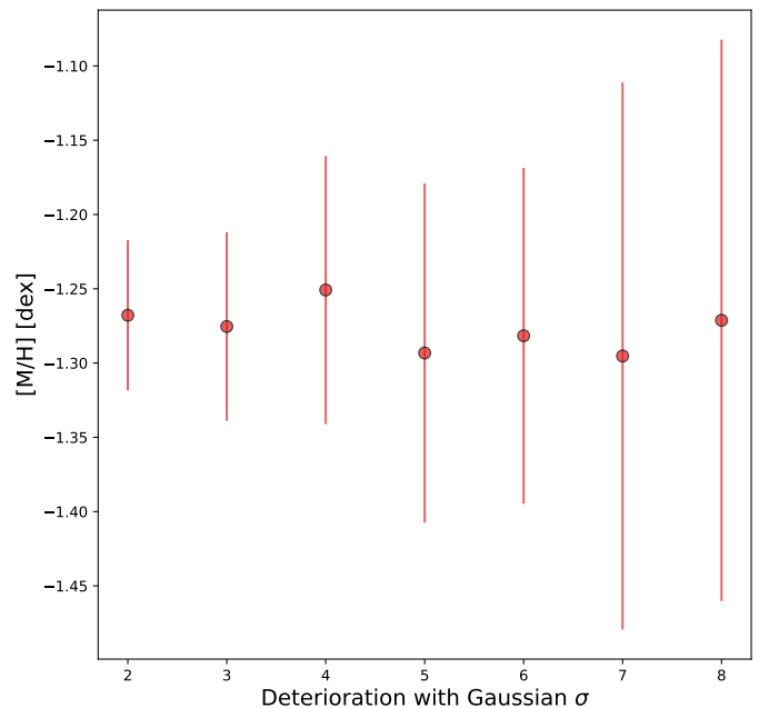
Fig. 11. Mean metallicity as a function of different degrees of spectrum deterioration for the highest S/N dwarf in the sample (MATLAS-553; S/N \sim 62 ). The error bars on the y -axis show the standard deviation of 100 MC realizations for every \sigma . The best-fit value for the metallicity is -1.29 dex.
