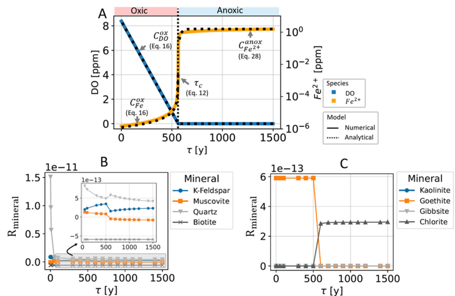
Figure 2. Simulation results for the Base Case scenario, obtained with Crunchflow for a lithological composition with \gamma_d = 2 \times 10^{-3} \text{ mol} \cdot \text{m}_{pm}^{-3} \cdot \text{y}^{-1} , \Lambda = 4 \times 10^4 . (a) Evolution of Dissolved Oxygen (DO) and iron concentration as a function of travel time ( \tau ). C_{DO}^{ox} and C_{Fe}^{ox} correspond to concentrations under oxic conditions, whereas C_{DO}^{anox} and C_{Fe}^{anox} represent concentrations at anoxic conditions. \tau_c is the characteristic time for DO depletion. (b and c) correspond to actual reaction rates for minerals ( R_{mineral} [\text{mol} \cdot \text{m}_{pm}^{-3} \cdot \text{s}^{-1}] ) as a function of fluid travel time for primary and secondary minerals, respectively.
