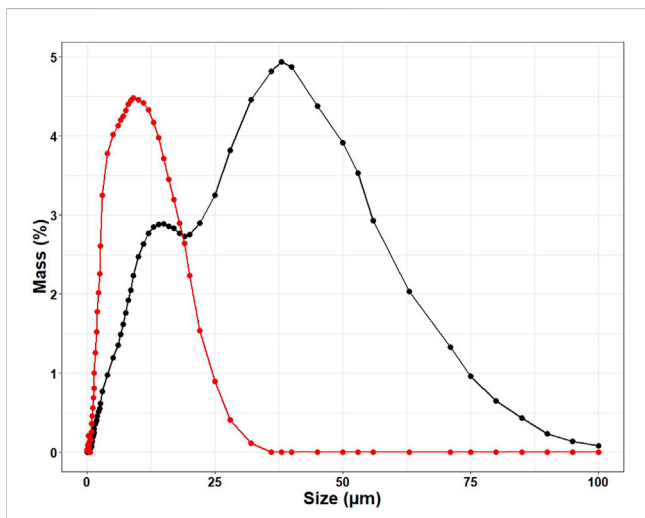
FIGURE 7 Particle-size distribution of suspended sediments at the Virey and Signy stations before the dams were removed.
