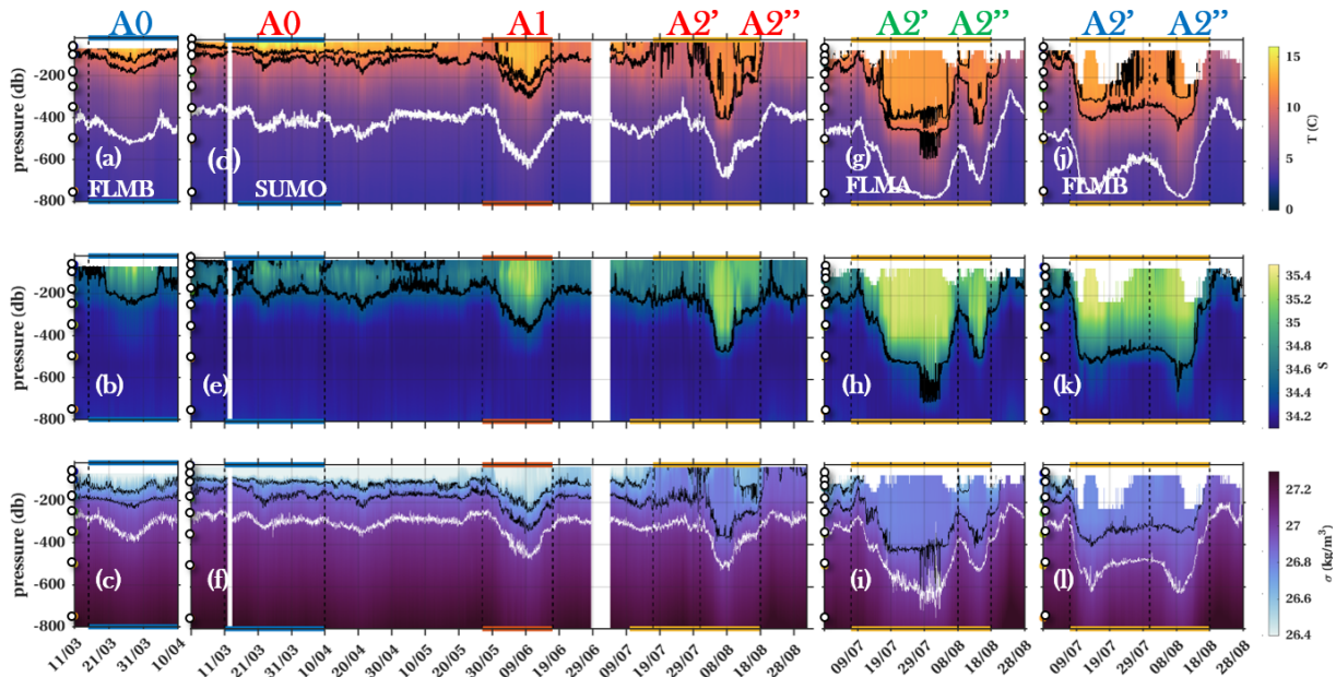
Figure 9. (a–c) Temperature, salinity and density from mooring B (FLMB) during A0 event (hourly averaged data are linearly interpolated in the vertical). In (a), the black isolines are 10°C and 12°C isotherms, and the white isoline is the 4.5°C isotherm. In (b), the black isoline is the 34.5 isohaline. In (c), the black isolines are the 26.65 and 26.85 kg m -3 isopycnals, and the white isoline is the 27.00 kg m -3 isopycnal. (d–f) Same as (a)–(c) at the surface mooring (SUMO) during events A0, A1 and A2. (g–i) Same as (a)–(c) at mooring A (FLMA) during event A2 event. (j–l) Same as (a)–(c) at mooring B (FLMB) during A2 event. White dots in the y axis indicate the discrete measurement levels.
