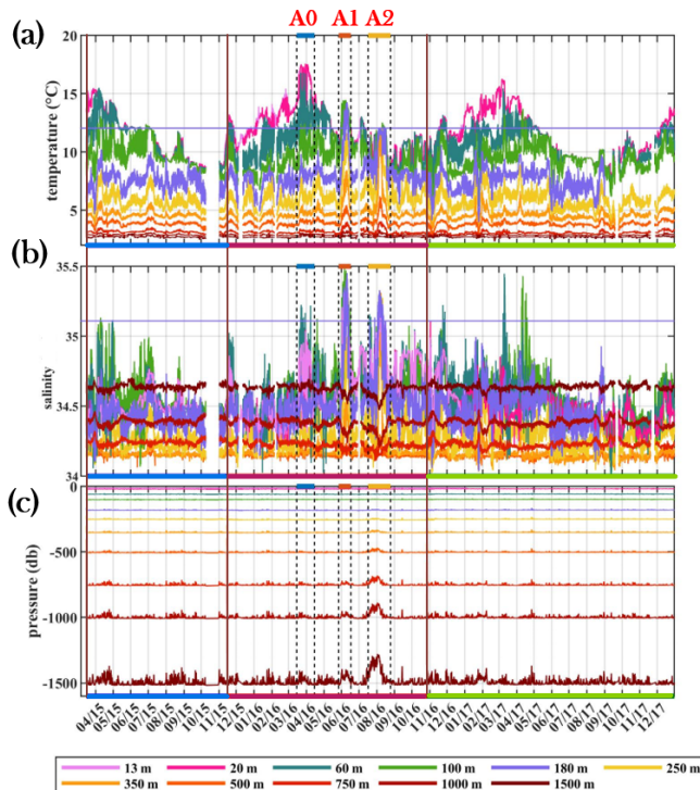
Figure 3. Temperature (a), salinity (b) and pressure (c) time series at the depths (indicated with colors) sampled at SUMO. The horizontal purple line in (a) (respectively (b)) corresponds to the mean plus 3 standard deviations of the temperature (respectively salinity) at 180 m. The color bars in the x axis delimit the three deployments: deployment 1 (blue), deployment 2 (red) and deployment 3 (green). Three events labeled A0, A1 and A2 stand out.
