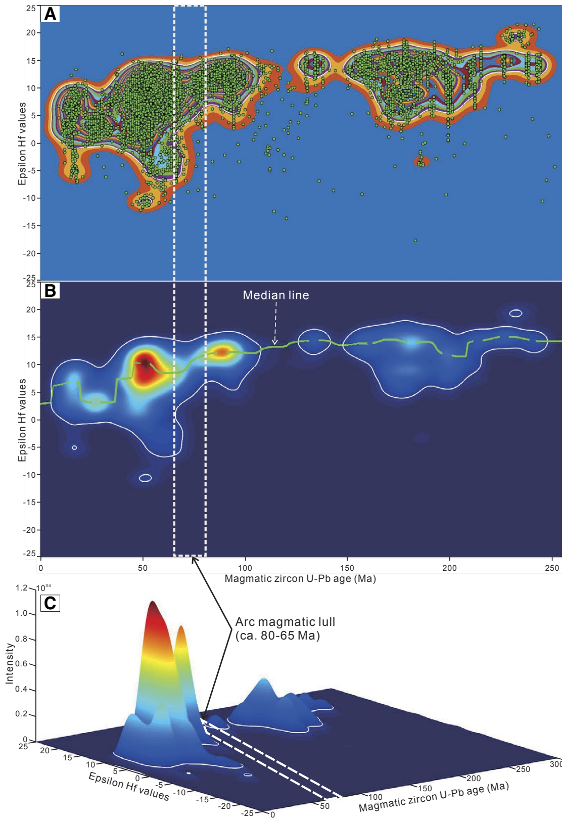
Figure 15. Distribution of magmatic zircon epsilon Hf values versus U-Pb ages (Ma). The magmatic zircon grains of igneous rocks were collected from the Gangdese magmatic belt, southern Tibet. The hafnium pattern plotting was complemented using the HafniumPlotter software (Sundell et al., 2019), which is a program designed for visualizing paired Lu-Hf geochemistry data—U-Pb geochronology as bivariate kernel density estimates (Botev et al., 2010; Sundell et al., 2019). A and B are 2-D intensity plots, while C is a 3-D intensity plot. A clearly shows the distribution of all samples, while B presents the clustering characteristics. The different colors in A represent different intensity, showing higher intensity to the core. The detailed Lu-Hf isotopic data of magmatic zircon grains from the Gangdese belt are listed in Table S7 (see text footnote 1).
