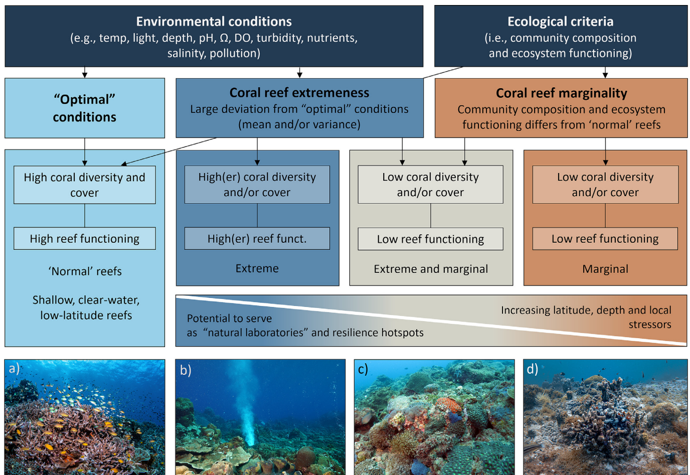
Fig. 1. A new classification framework to differentiate extreme versus marginal coral communities using environmental and ecological criteria. They are contrasted with ‘normal’ coral reefs that exist under optimal environmental conditions. Photos show illustrative examples of each type: (a) ‘normal’ coral reef in Indonesia (Credit: Brook Peterson | Ocean Image Bank), (b) extreme coral community near a CO 2 vent in Papua New Guinea (Credit: T. Shlesinger), (c) extreme and marginal high-latitude coral community at the Sunshine coast, Australia (Credit: B. Sommer), (d) marginal coral community surrounded by rubble and macroalgae, Curaçao, southern Caribbean (Credit: Lars ter Horst). For more examples, see Fig. S1. Note that extreme coral communities tend to have higher coral cover, diversity and reef functioning than marginal coral communities but these metrics may not be as high as on ‘normal’ reefs.
