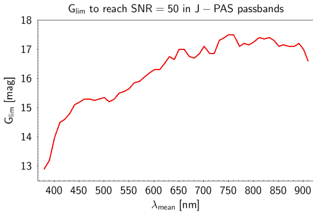
Fig. 19. G -band magnitude ( G_{lim} ) needed to reach a median S/N = 50 in every one of the narrow ( FWHM \sim 15 nm) J-PAS passbands with mean wavelength equal to \lambda_{mean} .
