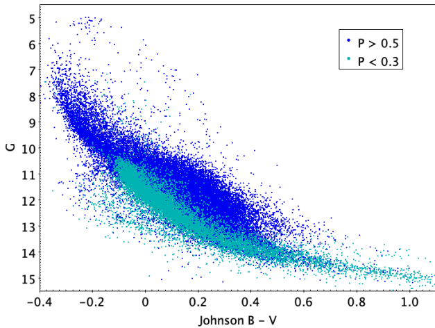
Fig. 45. (blue) Gaia absolute G magnitude vs. B-V colour–magnitude diagram for the GSPC-WD sample with probability of being a DA > 0.5 . (cyan) Gaia absolute G magnitude vs. B-V colour–magnitude diagram for the GSPC-WD sample with the probability of being a DA < 0.3 .
