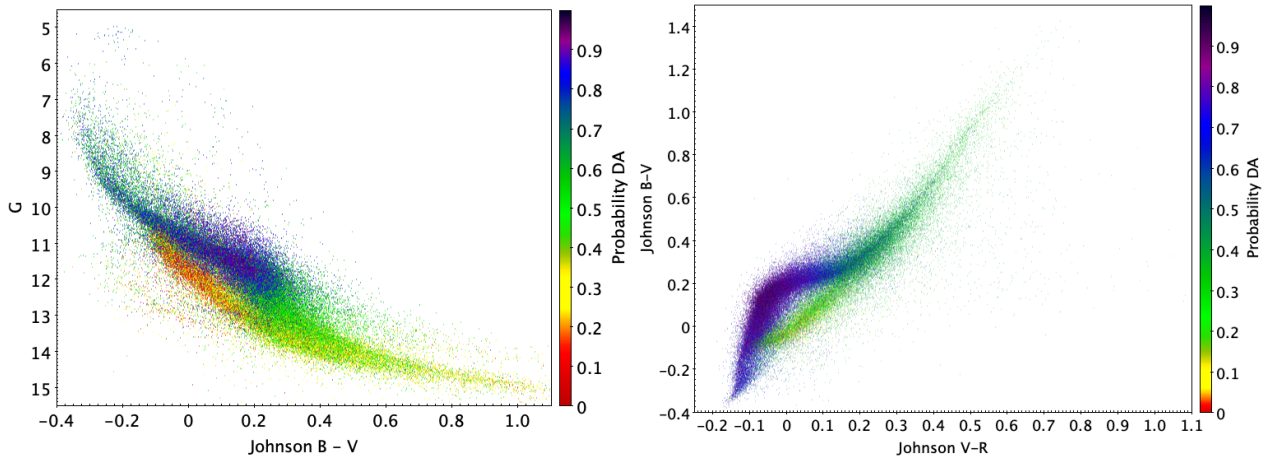
Fig. 44. (left) Gaia absolute G magnitude vs. B-V colour–magnitude diagram for the GSPC-WD sample colour-coded with the probability of a WD being a DA. (right) Gaia B-V vs. V-R colour–colour diagram for the GSPC-WD sample colour-coded according to the probability of a WD being a DA.
