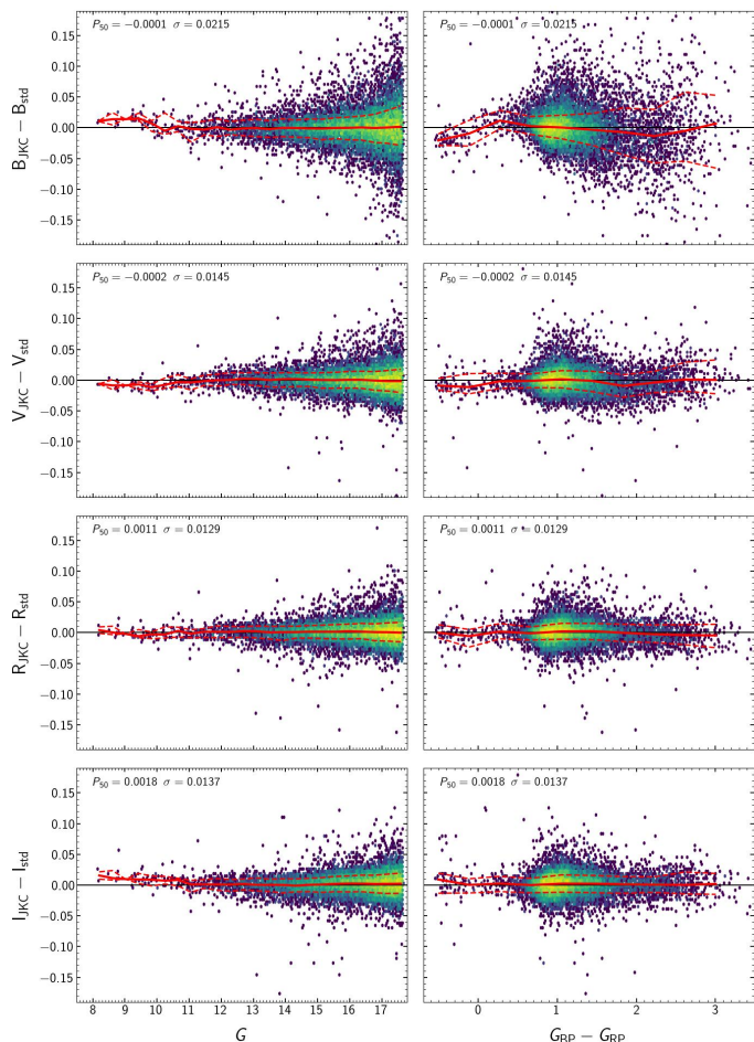
Fig. 10. Performances of standardised XPSP in the JKC system ( BVRI ). We show \Delta\text{mag} as a function of G magnitude (left panels) and G_{\text{BP}} - G_{\text{RP}} colour (right panels) for the subsample of reference stars whose XP spectra has been released in Gaia DR3. The arrangement and the meaning of the symbols is the same as in Fig. 6.
