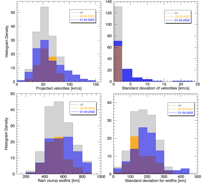
Fig. 18. Projected velocities (top), widths (bottom), and associated standard deviation (corresponding to the right panels) for all rain clumps. The colours include transparency and denote different dates (see legends).
