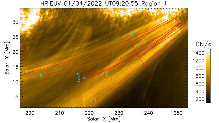
Fig. 10. Close-up of the footpoint of a large coronal loop bundle observed on 2022 April 1st by HRI EUV . The FOV corresponds to that of region 1 indicated by the white rectangle in the right panel of Fig. 1. Except for path 8 (which crosses the loop bundle), the red paths denote several rain paths. An animation of this figure is available online , whose images have been processed with the wavelet-optimised whitening enhancement technique of Auchère et al. (2023). It runs from UT 09:19 to UT 10:34 and shows several rain clumps falling towards the chromosphere. The movie first runs without and then with the rain paths overlaid.
