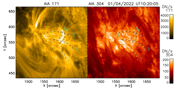
Fig. 21. SDO/AIA observation in the 171 (left) and 304 (right) channels of the April 1st coronal rain events. AIA was roughly in quadrature with Solar Orbiter on this date. Some of the large loop bundles observed by HRI EUV can be easily identified. The dashed white-black paths follow some rain clumps belonging to these loop bundles that are observed in AIA 304. Path 1 follows the same loop bundle as in region 1 of Fig. 10. Paths 2 and 3 may correspond to the same rain events that were shown in paths 8 or 9 in region 2 of Fig. 11. Paths 4 and 5 follow the same loop bundle as was shown in the lower part of Fig. 13 (paths 1 to 6 in that figure). An animation corresponding to this figure is available online . The animation shows widespread rain in AIA 304, but the counterparts in AIA 171 can only clearly be seen for the loop around path 1, although strong intensity variations are observed at the same locations. The animation runs from UT 09:20 to UT 10:32 and comprises the time where coronal rain is observed with HRI EUV . It first runs without and then with the rain paths overlaid.
