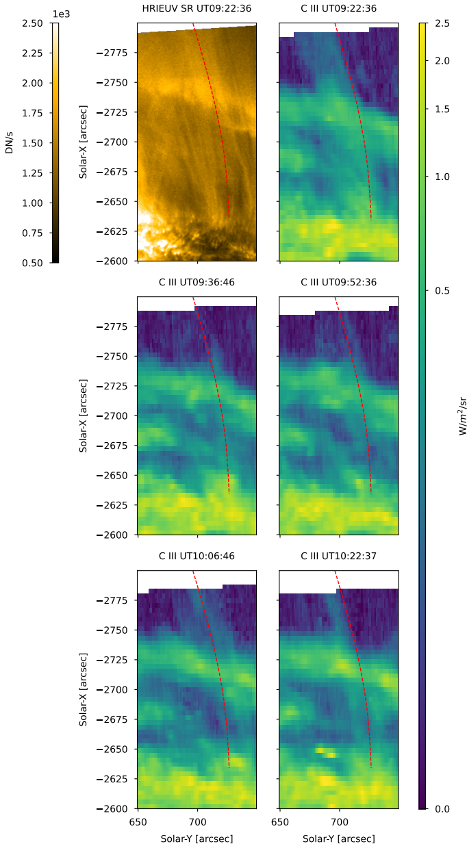
Fig. 17. SPICE rasters in the C III line ( \log T = 4.8 K) over a region that overlaps with region 4 on April 1st. The FOV corresponds to the red rectangle to the east shown in Fig. 2 (bottom), and the overlaid red curves denote some of the rain paths seen with HRI EUV (see Figs. 10 and 11). The HRI EUV panel corresponds to an SR matching the time of the first SPICE raster (see the text for details), but preserving the HRI EUV spatial resolution. The SPICE panels show the total intensity integrated over the C III spectral line for each raster (the time is shown in the subtitle).
