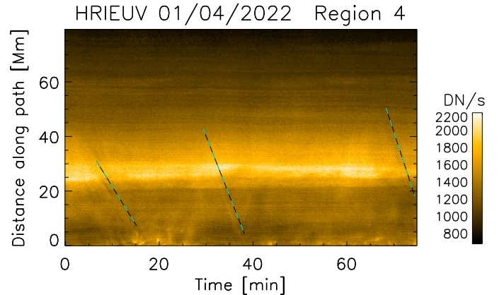
Fig. 16. Time-distance diagram along a loop observed partly off-limb by \text{HRI}_{\text{EUV}} on April 1st. The path corresponds to red curve in region 4 shown in Fig. 1. The dashed cyan and black lines correspond to dark and bright tracks from coronal rain (offset in time by 1 min in the figure for clarity).
