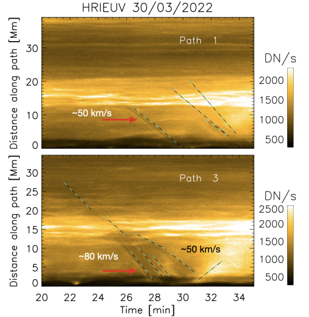
Fig. 8. Time-distance diagrams along paths 1 and 3 indicated in Fig. 5. The distance increases with height along the paths. The dark tracks traced by the dashed cyan-black lines correspond to EUV absorption from falling rain clumps. The dashed lines are offset by a fraction of a minute so that the rain features appear more clearly. An estimate of the projected velocity is given for the closest slope to each value. We note the bright tracks that are indicated by the red arrows immediately beneath the first dark tracks in each diagram. We interpret this feature as compression and heating from the clump. We interpret the upward bright and diffuse slope at the end of the time sequence ( t \approx 30 – 32 min) in path 3 as a combination of a rebound shock and flow produced by the rain impact on the chromosphere.
