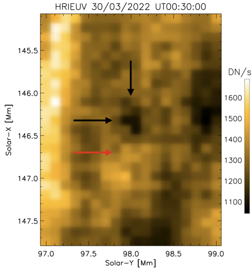
Fig. 7. Close-up of the sub-FOV indicated by the white rectangle in Fig. 5. The dark feature indicated by the arrows corresponds to the EUV absorption produced by a rain clump. We interpret the bright feature below (downstream of) the rain clump indicated by the red arrow as compression and heating produced by the rain clump as it falls.
