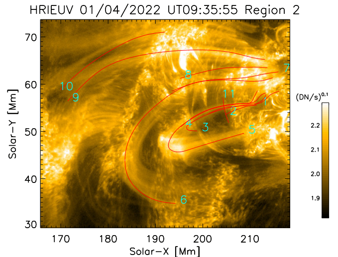
Fig. 11. FOV corresponding to region 2, shown in Fig. 1 (right panel). The red curves correspond to paths of some of the observed coronal rain clumps. We note that the intensities are scaled with a power of 0.1 to show a wider range of variations. An animation of this figure is available online , whose images have been processed with the wavelet-optimised whitening enhancement technique of Auchère et al. (2023). It runs from UT 09:19 to UT 10:34 and shows several rain clumps falling towards the chromosphere. The movie first runs without and then with the rain paths overlaid.
