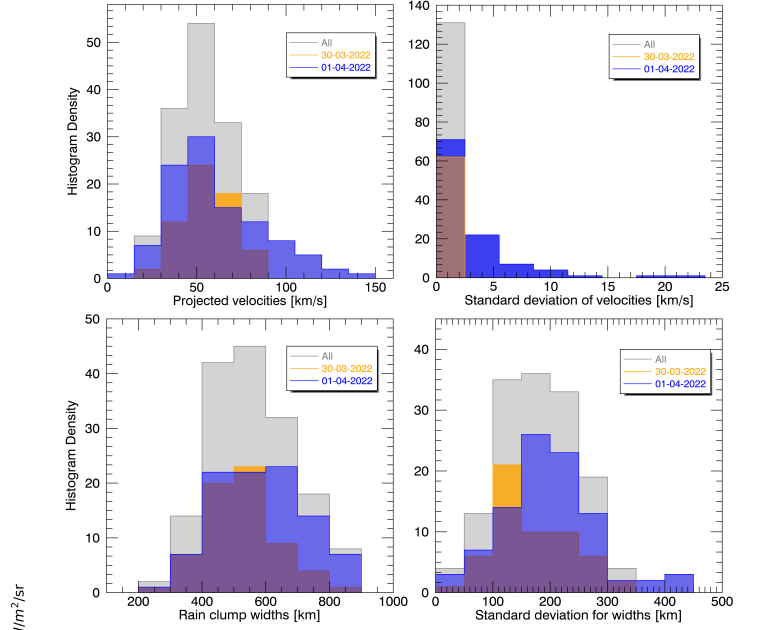
Fig. 18. Projected velocities (top), widths (bottom), and associated standard deviation (corresponding to the right panels) for all rain clumps. The colours include transparency and denote different dates (see legends).
