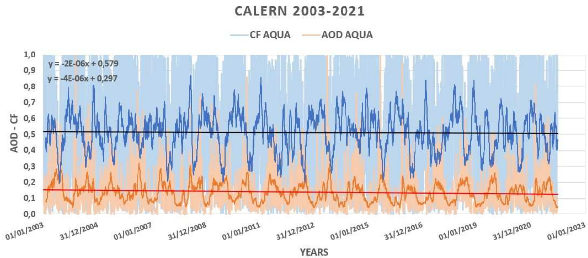
Figure 4. Trends of the daily time series of CF and AOD (Aqua, 2003-2021), with their respective 30-day moving averages and linear regressions, measured by MODIS-Aqua at the Calern site. The y-axis simultaneously indicates the cloud cover fraction (CF) and the aerosol optical depth (AOD). The equations of the regression lines and its angular coefficient ( M ) in the upper left provide an estimate of the long-term trend of cloud cover ( M_{CF} = -2.0 \cdot 10^{-6} \text{ day}^{-1} ) and aerosols ( M_{AOD} = -4.0 \cdot 10^{-6} \text{ day}^{-1} ).
