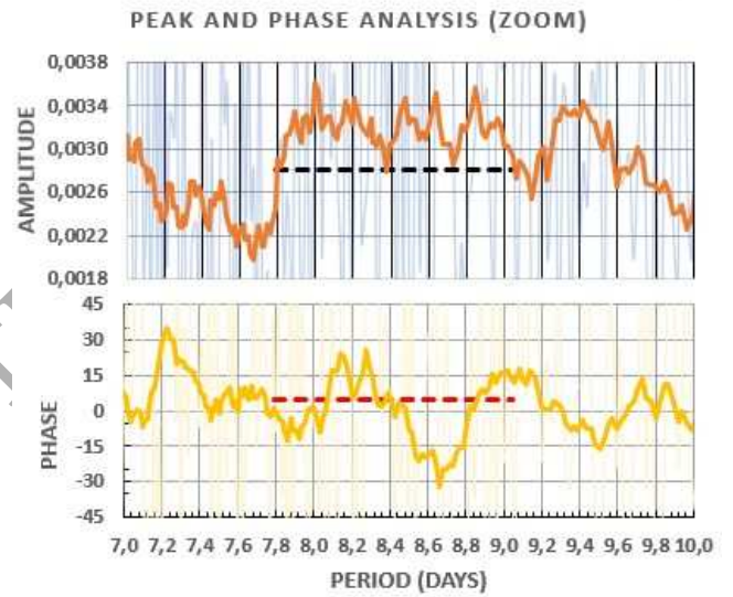
Figure 7. Analysis of the peak periodicity (P1-Figure 6 Zoom) for the amplitude (top panel) and the phase (bottom panel). FWHM represents signal dispersion (dashed line - top panel). Phase is derived from the average phase bounded by the dotted line in the bottom panel
