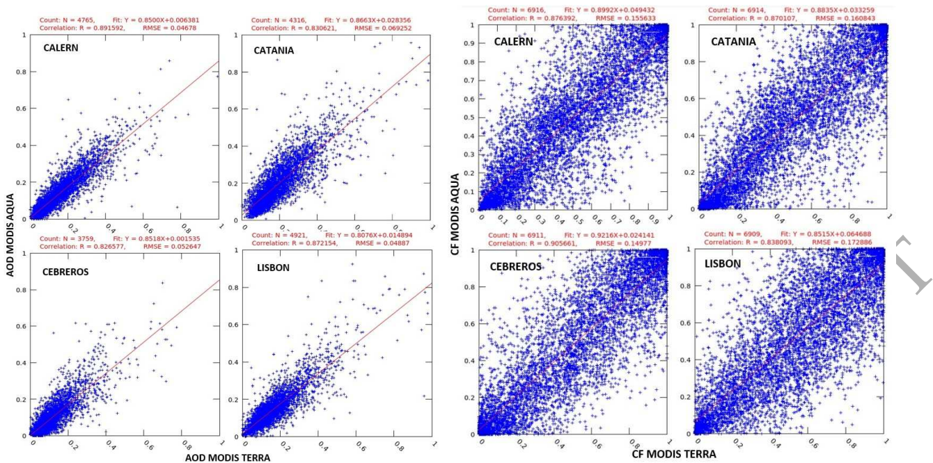
Figure 10. AOD (left panel) and CF (right panel) MODIS Terra-Aqua (2003-2021) correlation at the four candidate sites of the ANAtOLIA project.
