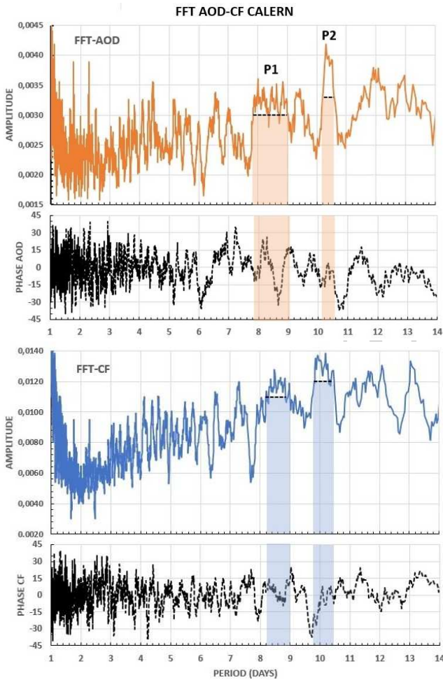
Figure 6. FFT of the MODIS-Aqua AOD and CF time series (2003-2021) at the Calern site (Top panel: amplitude; bottom panel: phase in degrees).
