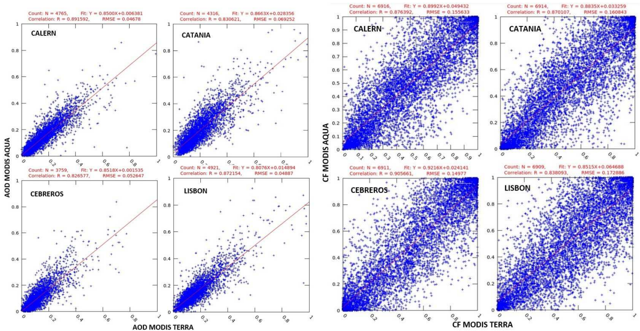
Figure 10. AOD (left panel) and CF (right panel) MODIS Terra-Aqua (2003-2021) correlation at the four candidate sites of the ANAtOLIA project.
