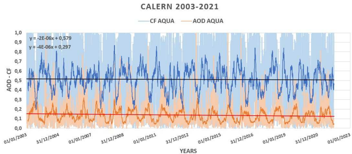
Figure 4. Trends of the daily time series of CF and AOD (Aqua, 2003-2021), with their respective 30-day moving averages and linear regressions, measured by MODIS-Aqua at the Calern site. The y-axis simultaneously indicates the cloud cover fraction (CF) and the aerosol optical depth (AOD). The equations of the regression lines and its angular coefficient ( M ) in the upper left provide an estimate of the long-term trend of cloud cover ( M_{CF} = -2.0 \cdot 10^{-6} \text{ day}^{-1} ) and aerosols ( M_{AOD} = -4.0 \cdot 10^{-6} \text{ day}^{-1} ).
