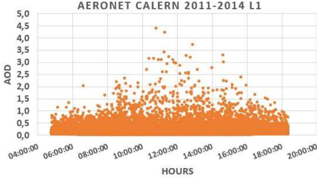
Figure 8. Hourly percentile analysis from AERONET data at the Calern site (2011-2014). The dots show the daily trend of concentrated aerosols between 10:00 and 15:00 (local solar time).
