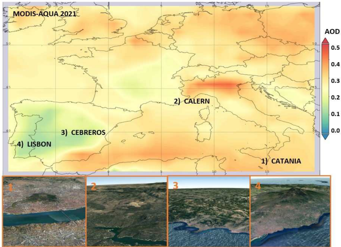
Figure 1. Location of the four sites involved in the analysis on the annual AOD time average map measured by Aqua satellite in 2021. As seen in the inserts the selected sites presents very different topographic conditions.
