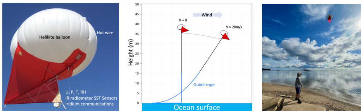
Fig. 14. Pictures and schematic of the Aeroclipper System. (left and middle): design and measurement principle, (right) Aeroclipper released from Guam in September 2022. Credit: Jean-Philippe Duvel.
