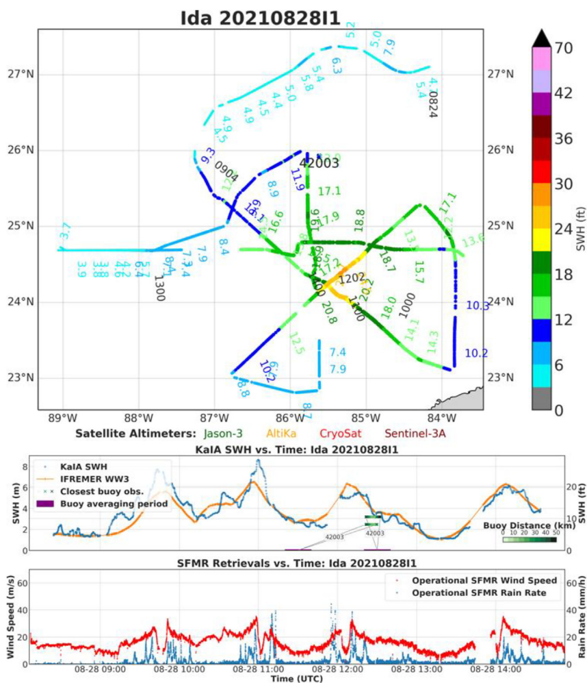
Fig. 6. KaIA significant wave height data collected during a flight into Hurricane Ida on August 28, 2021 plotted along the flight track (top) and as a time series (middle) as well as the corresponding IFREMER forecast significant wave height and SFMR wind speed and rain rate (bottom).
