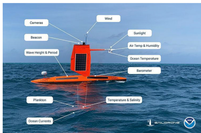
Fig. 12. Picture of the extreme weather Saildrone uncrewed surface vehicle and its suite of different sensors. Credit: NOAA and Saildrone Inc., ©2021.
