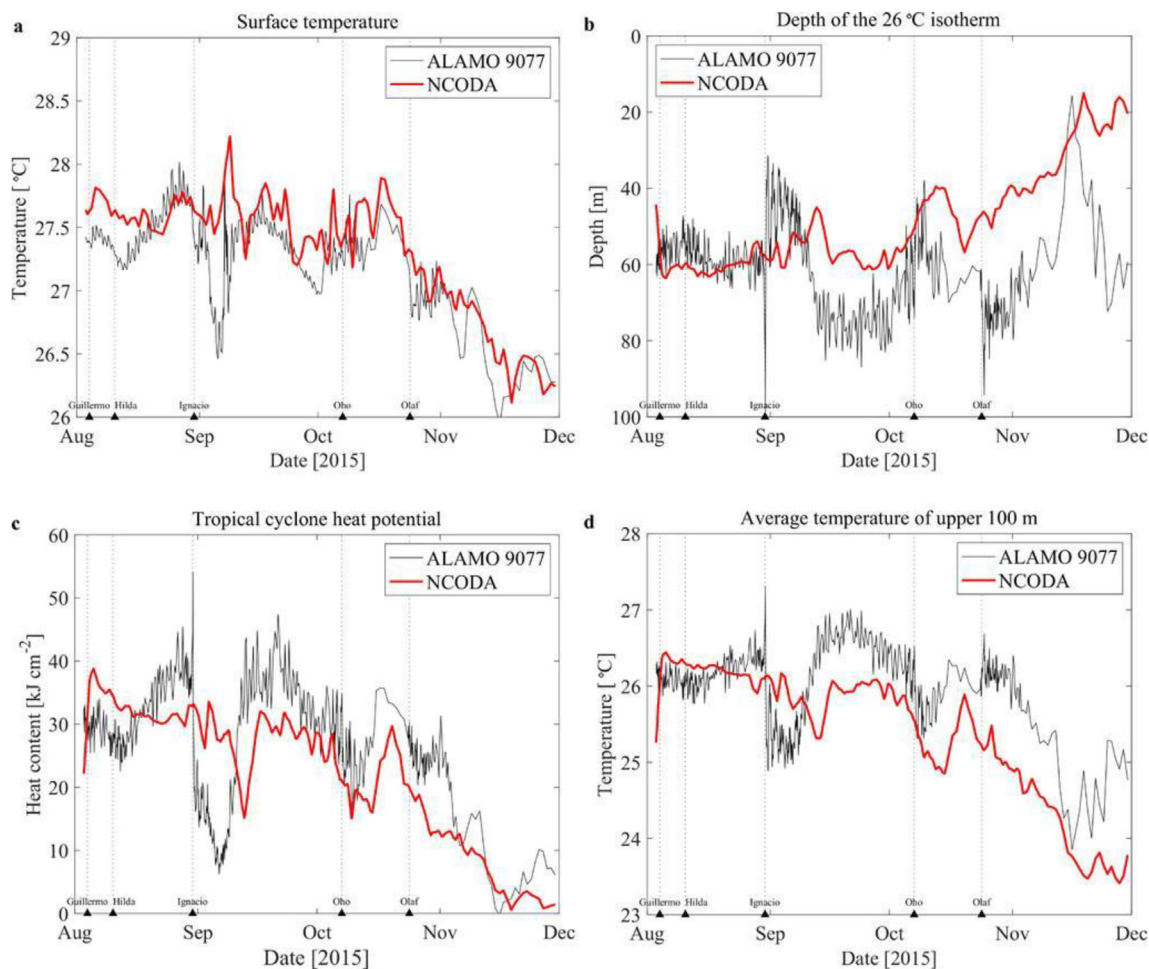
Fig. 9. Metrics comparing the NCODA analysis to observations from the ALAMO float 9077 deployed ahead of Hurricane Guillermo (Eastern Pacific) in 2015: (a) the sea surface temperature ( ^{\circ}\text{C} ), (b) depth of the 26^{\circ}\text{C} isotherm (m), (c) TC heat potential ( \text{kJ cm}^{-2} ), and (d) average temperature of the upper 100 m ( ^{\circ}\text{C} ). Small triangles with gray dotted lines and TC names along the time axis indicate the time of closest point of approach between the float and each storm. Reproduced from Jayne et al. (2022).
