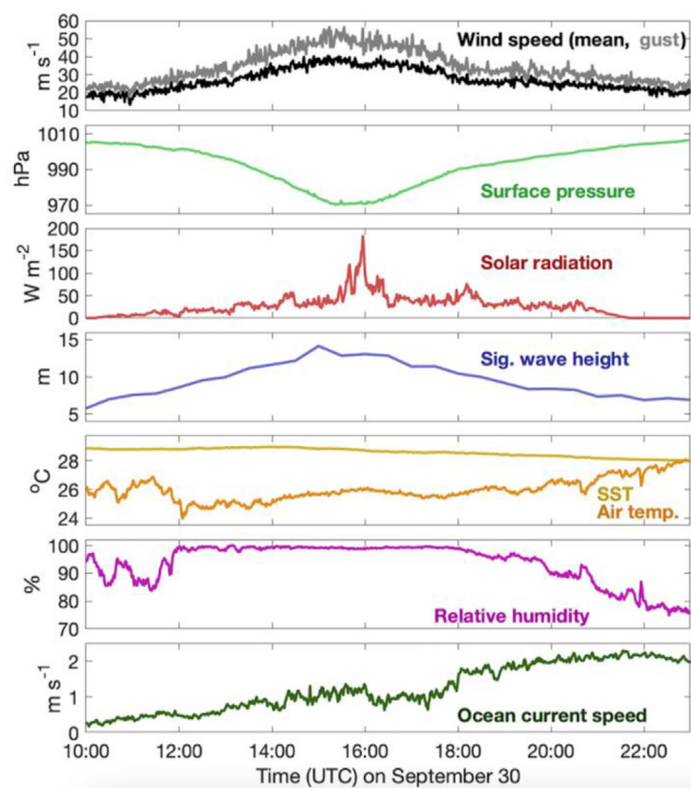
Fig. 13. 1-min averaged data of wind speed ( \text{m s}^{-1} ), surface air pressure (hPa), solar radiation ( \text{W m}^{-2} ), significant wave height, sea surface and air temperatures, relative humidity, and ocean current speed at a depth of 6 m, as measured by SD-1045 in Hurricane Sam. Reproduced from Foltz et al. (2022).
