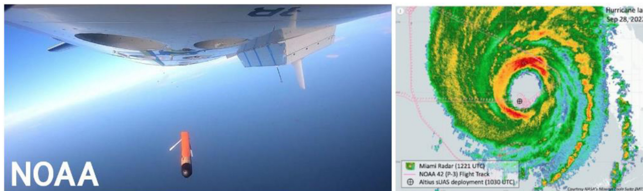
Fig. 11. (a) The Area-I's Altius 600 sUAS being deployed from one of the two NOAA P-3 aircrafts. (b) Location of the drone into the eye of Hurricane Ian superimposed on radar reflectivity on September 28, 2022. Credit: NOAA.
