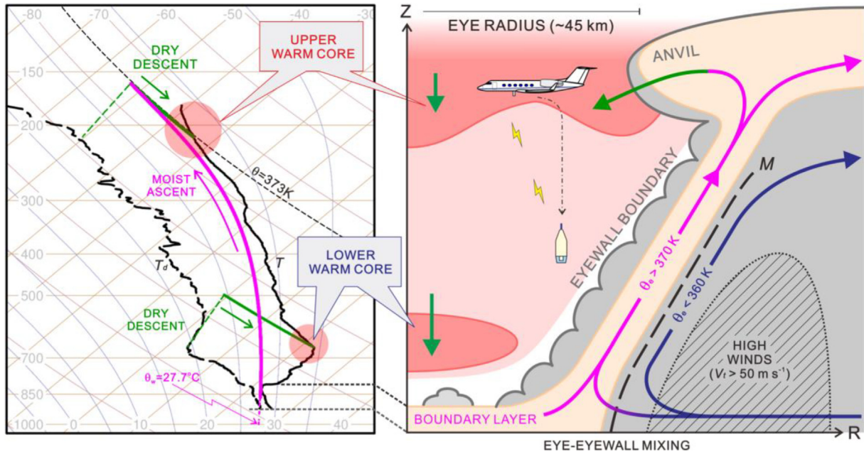
Fig. 3. Schematic view of the double warm cores observed for Typhoon Lan (2017). Reproduced from Yamada et al. (2021).
