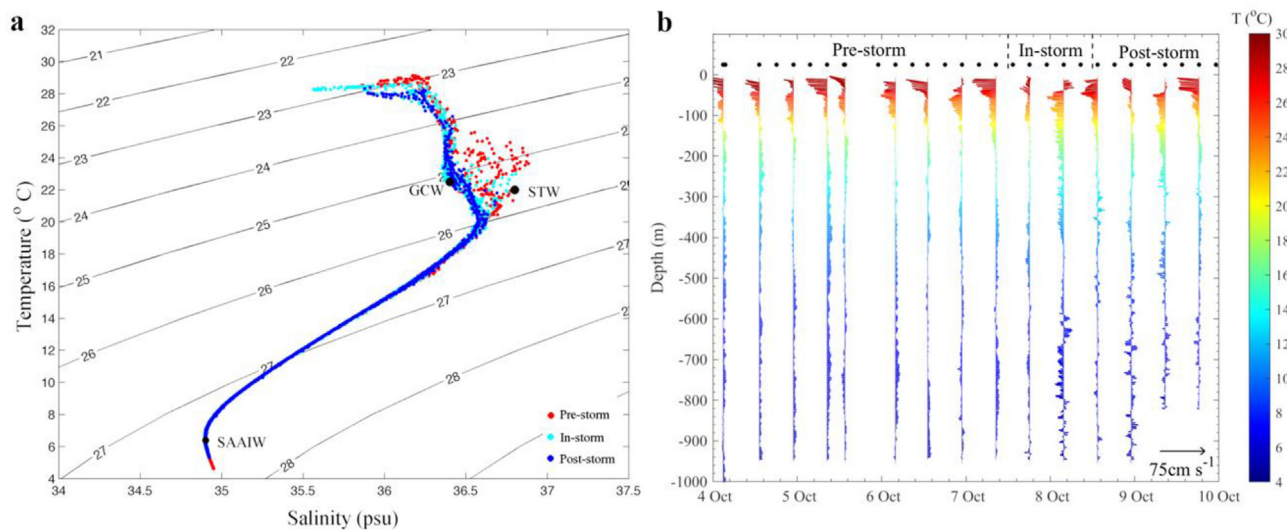
Fig. 8. Temperature and salinity measurements (left panel) and current profile measurements (right panel) from an APEX-EM float deployed in Hurricane Nate (2017) over a warm core eddy. Red, light blue, and dark blue profiles signify pre-, in-, and post-storm measurements, respectively. GCW, STW, and SAAIW stand for Gulf Common Water, Subtropical Water, and Sub Antarctic Intermediate Water in the left panel. Velocity profiles (color coded by temperature) were obtained at each black dot (for clarity in the presentation, every other profile is shown). Reproduced from Shay et al. (2019).
