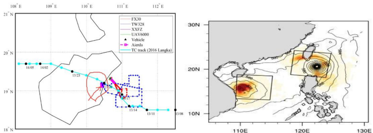
Fig. 4. (left panel): Typhoon “Nangka” (No. 2016) multi-platform collaborative observation drone detection route and typhoon path. (right panel): The target observation sensitive areas of Typhoons “Conson” and “Chanthu”, which are shown in the black box near the center of the typhoon.
