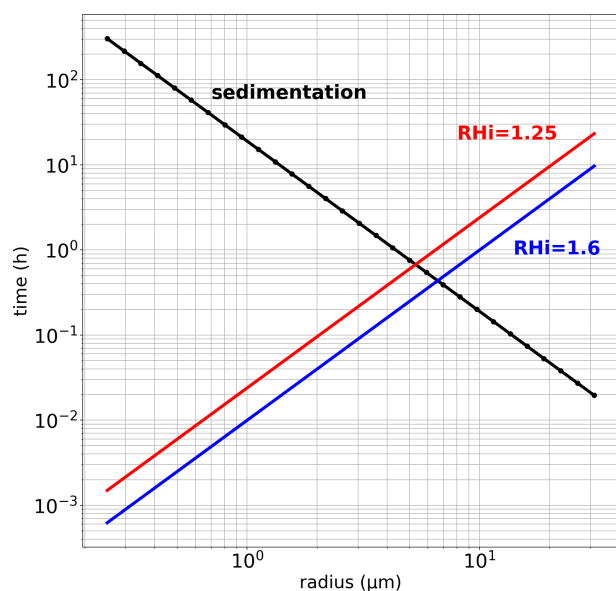
Figure 5. Typical timescales of ice-crystal (black) sedimentation, (red) \text{RH}_i = 1.25 , and (blue) \text{RH}_i = 1.6 growth rates, depending on their size.
