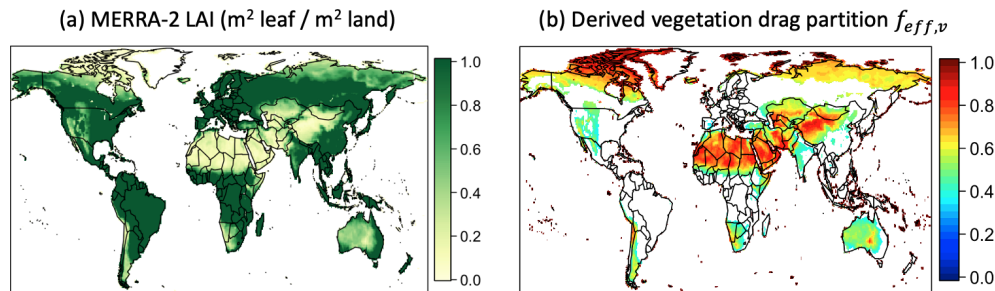
Figure 3. Vegetation drag partition factor f_{\text{eff},v} derived from the Okin (2008) and Pierre et al. (2014) drag partition model for the year 2006 on a 0.5^\circ \times 0.625^\circ grid. (a) Annual mean MERRA-2 LAI, with color bar saturated at a value of 1. (b) Annually averaged f_{\text{eff},v} derived using the Okin (2008) and Pierre et al. (2014) drag partition model. White areas indicate water body, ice/snow, or LAI > 1.
