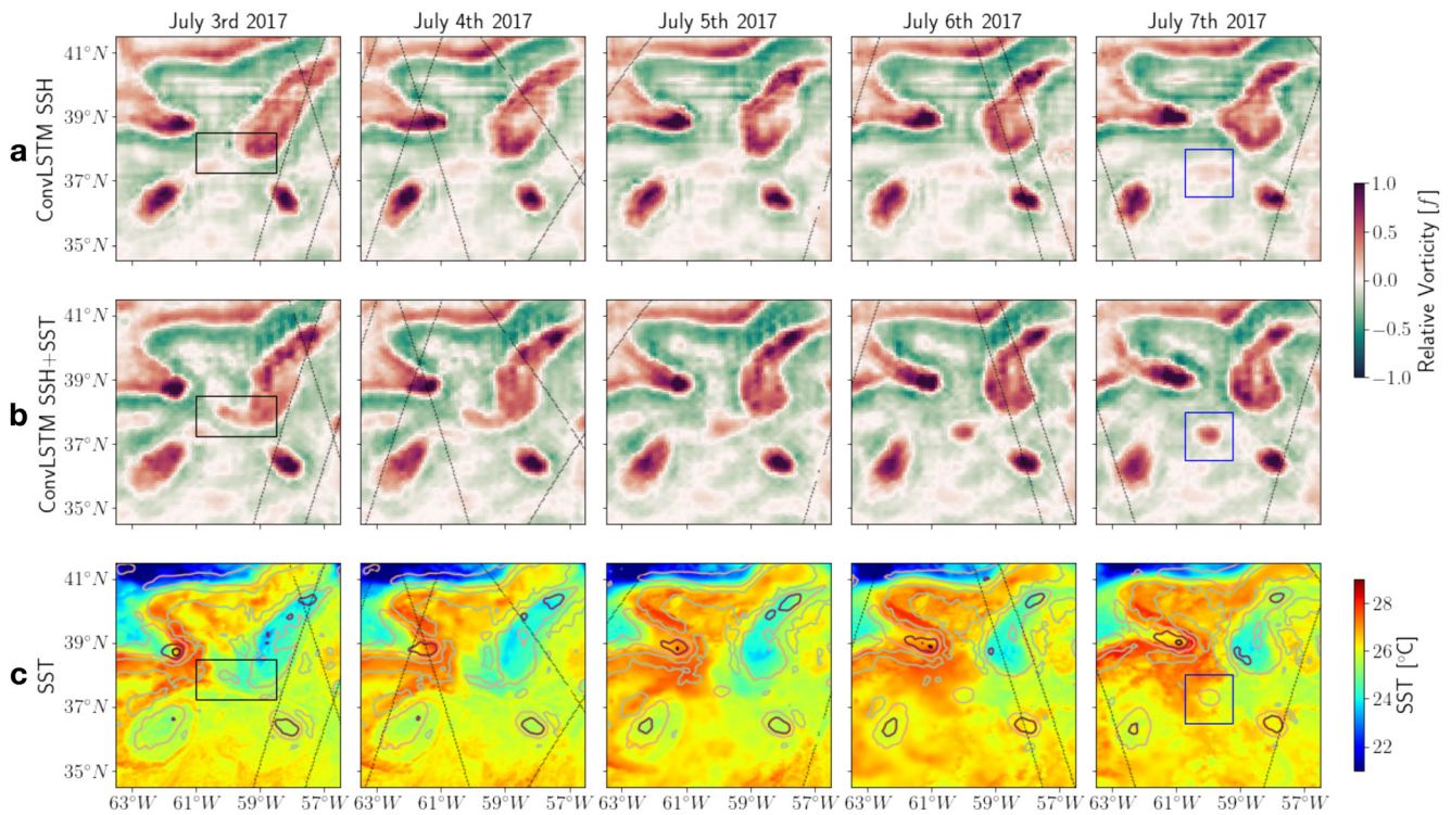
Figure 14. Relative vorticity from (a) the ConvLSTM SSH and (b) the ConvLSTM SSH + SST reconstructions for 5 consecutive days. GHRSSST Multiscale Ultra-high-Resolution SST for the same days is shown in row (c) and the locations of the satellite altimetry observations on each day are overlaid in black. ConvLSTM SSH + SST relative vorticity contours in increments of 0.5f from -1.25f to 1.25f are overlaid over the SST observations. The black box on July 3rd highlights the filament from which this eddy formed.
