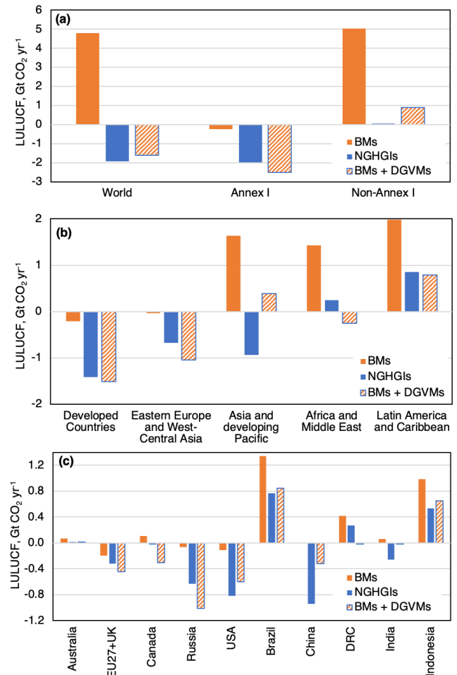
Figure 7. LULUCF CO 2 fluxes (average 2000–2020) from BM, from the sum of BM and DGVM (in non-intact forest only) and from NGHGI, for the world, Annex I countries (AI), and Non-Annex I countries (NAI, panel a) and for five macro-regions (b) and for 10 large individual countries (c).
