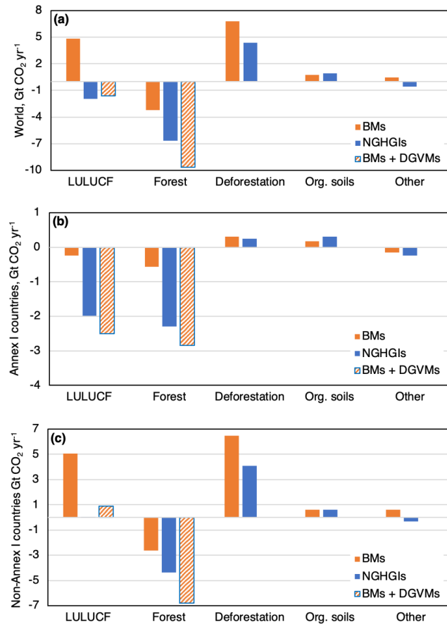
Figure 8. Land CO 2 fluxes (average 2000–2020) from BMs, from the sum of BMs and DGVMs (in non-intact forest only) and from NGHIGs for the total LULUCF sector, forest land (including harvested wood products and excluding organic soils), deforestation, organic soils and other (cropland, grassland, etc.) at the global level (panel a), for Annex I countries (b), and for Non-Annex I countries (c).
