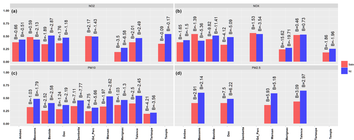
Figure 13. Statistics for the comparisons of measurements performed at air quality stations for NO 2 , NO x , PM 10 , and PM 2.5 in the simulations. The y axis shows the correlation coefficient, while the bias (simulation–observation) for each station is written on each bar. The comparisons involve the base case (in red) and the final test case (in blue).
