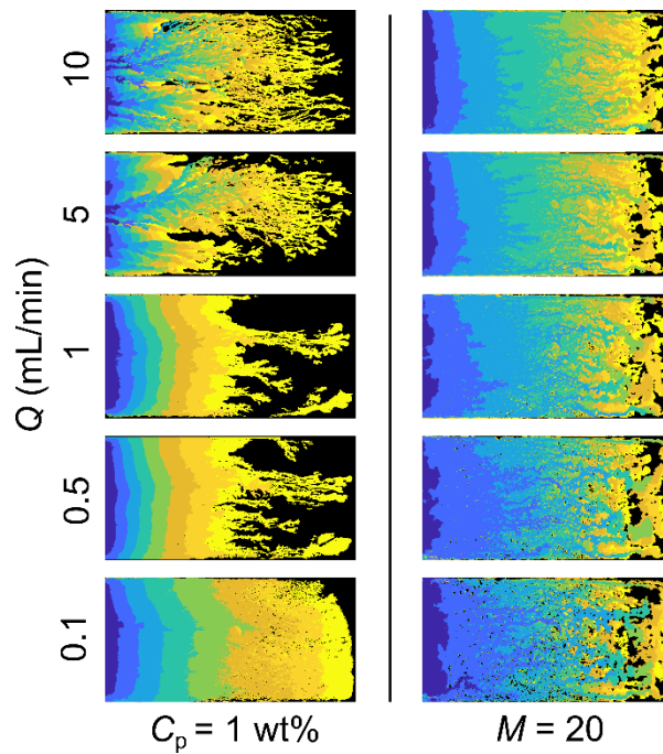
Figure 6. Evolutions of the fluid-fluid displacement fronts with time under shear-thinning fluid (Xanthan solutions) invading and Newtonian fluid (water-glycerol mixtures) invading conditions. The blue color represents the initial stage and the yellow indicates late times.
